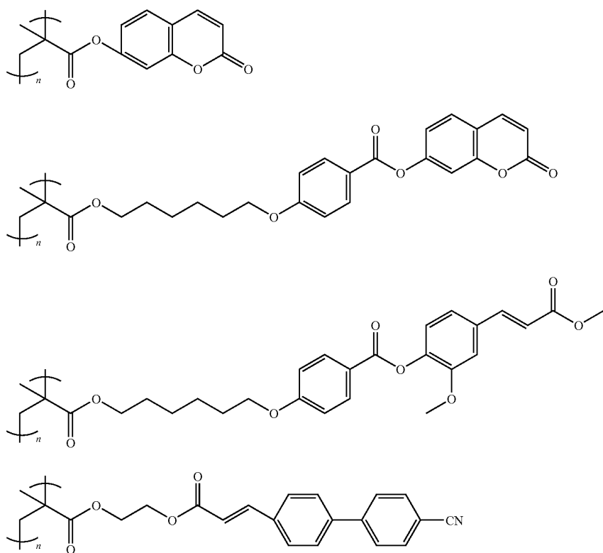
[Chemical Formula 8]
