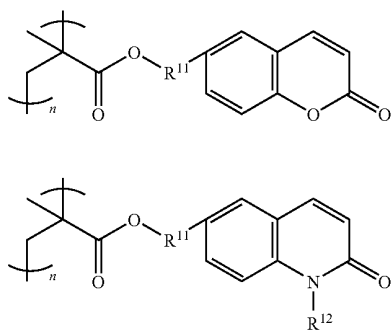
[Chemical Formula 7]
