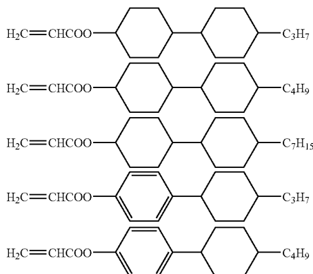
[Chemical Formula 2]
