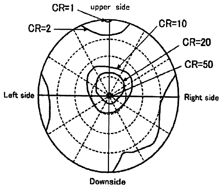
FIG.2A(PRIOR ART)
