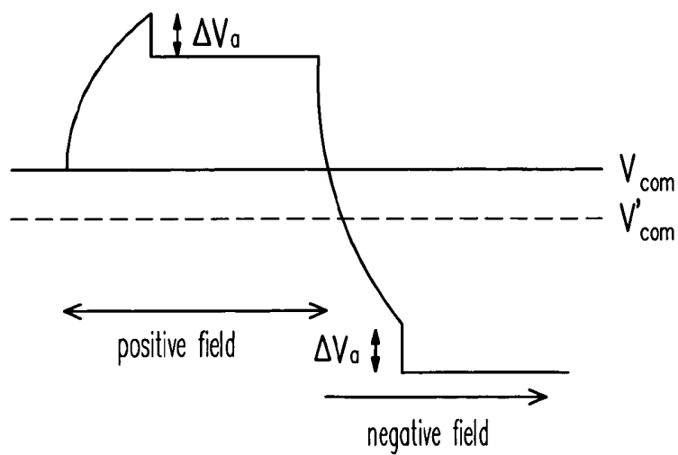
FIG. 5 (PRIOR ART)
