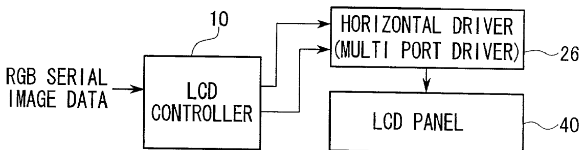
FIG. 3B WHEN A DRIVER IS ARRANGED AT ONE SIDE OF LCD PANEL
