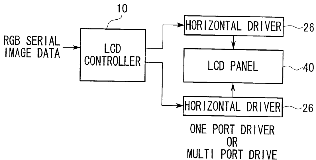
FIG. 3A WHEN DRIVERS ARE ARRANGED AT BOTH SIDES OF LCD PANEL
