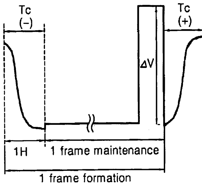
FIG. 5 CONVENTIONAL ART
