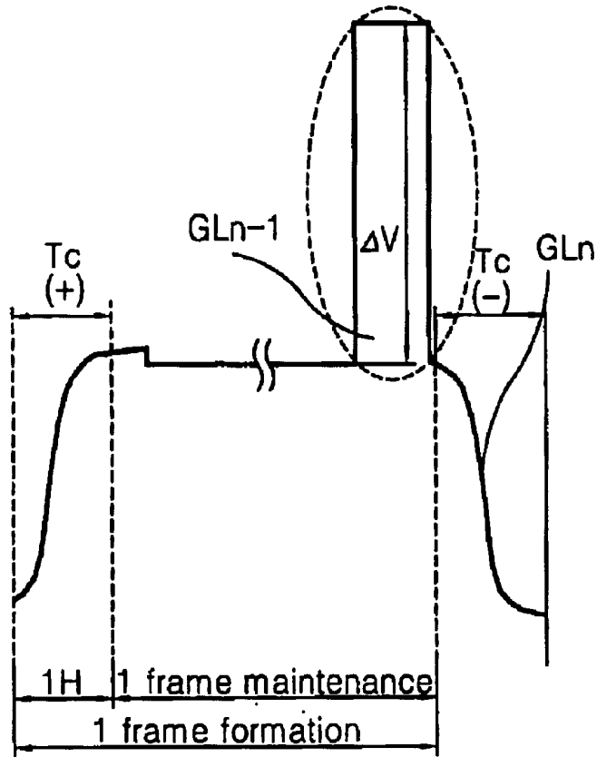
FIG. 4 CONVENTIONAL ART
