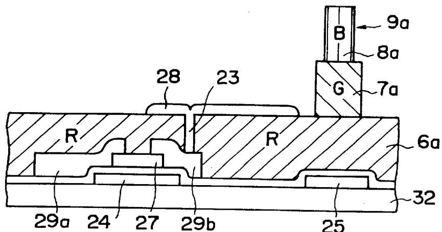
X1-X1' CROSS SECTION
