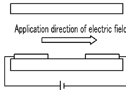
Application state of electric field birefringence
