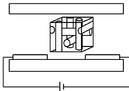
Absence state of electric field blue phase and non-birefringence
