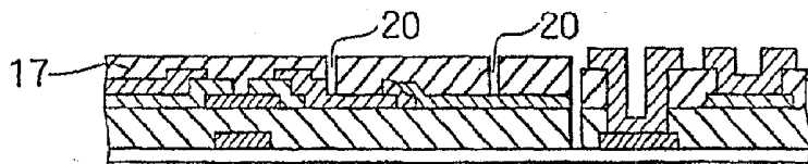
FIG. 13D
