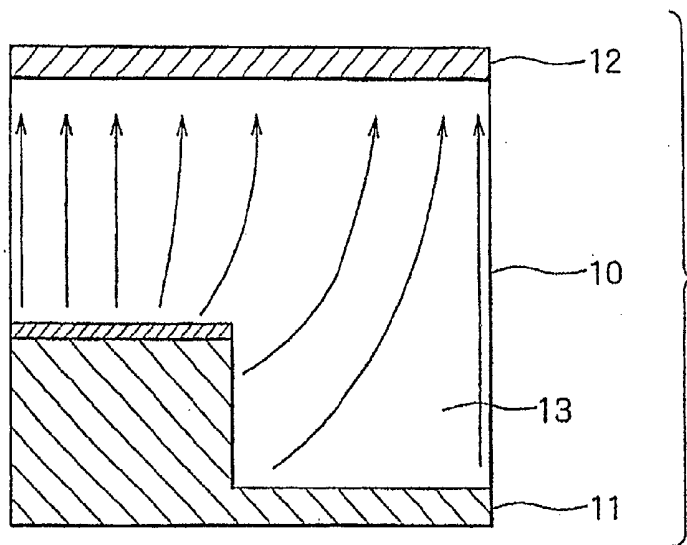
FIG. 3 (PRIOR ART)
