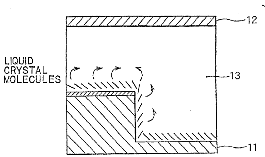
FIG. 4 (PRIOR ART)
