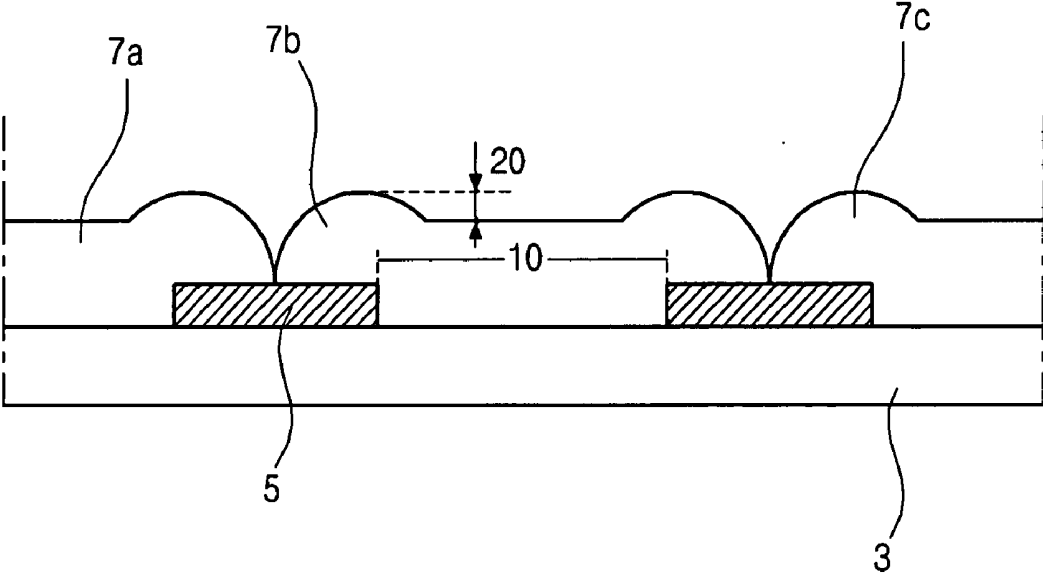
FIG. 2C Related Art
