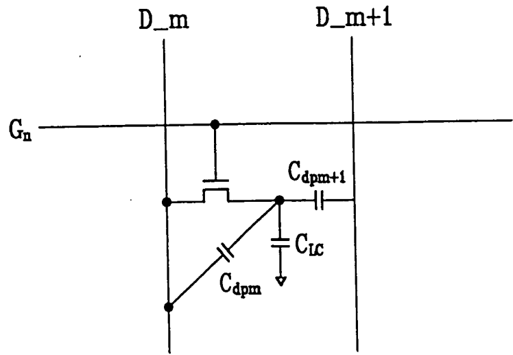
FIG. 4 Related Art
