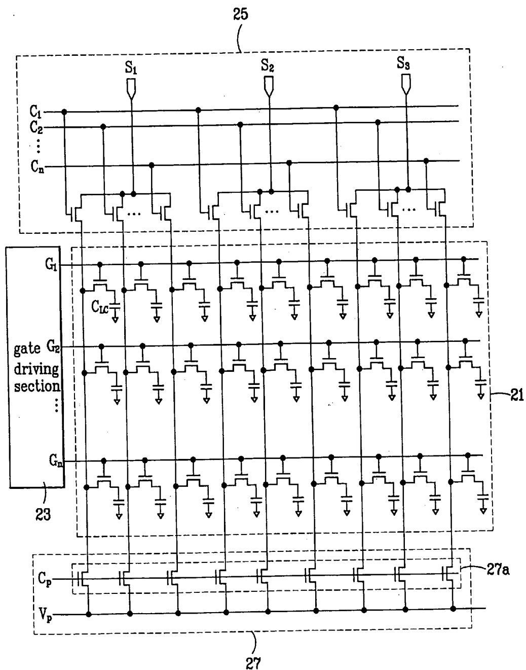
FIG.2 Related Art
