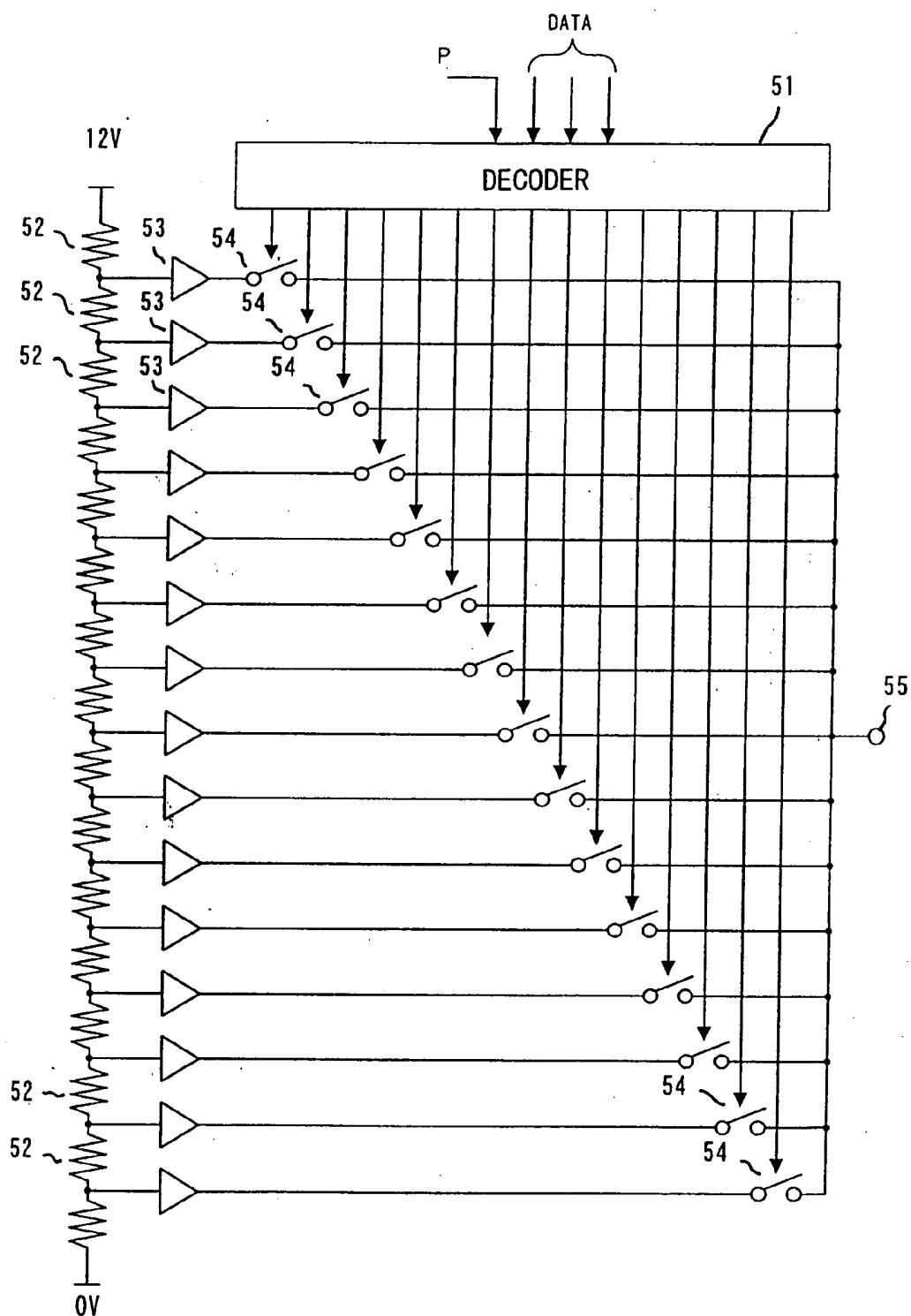
CONFIGURATION OF D/A CONVERTER 46a
