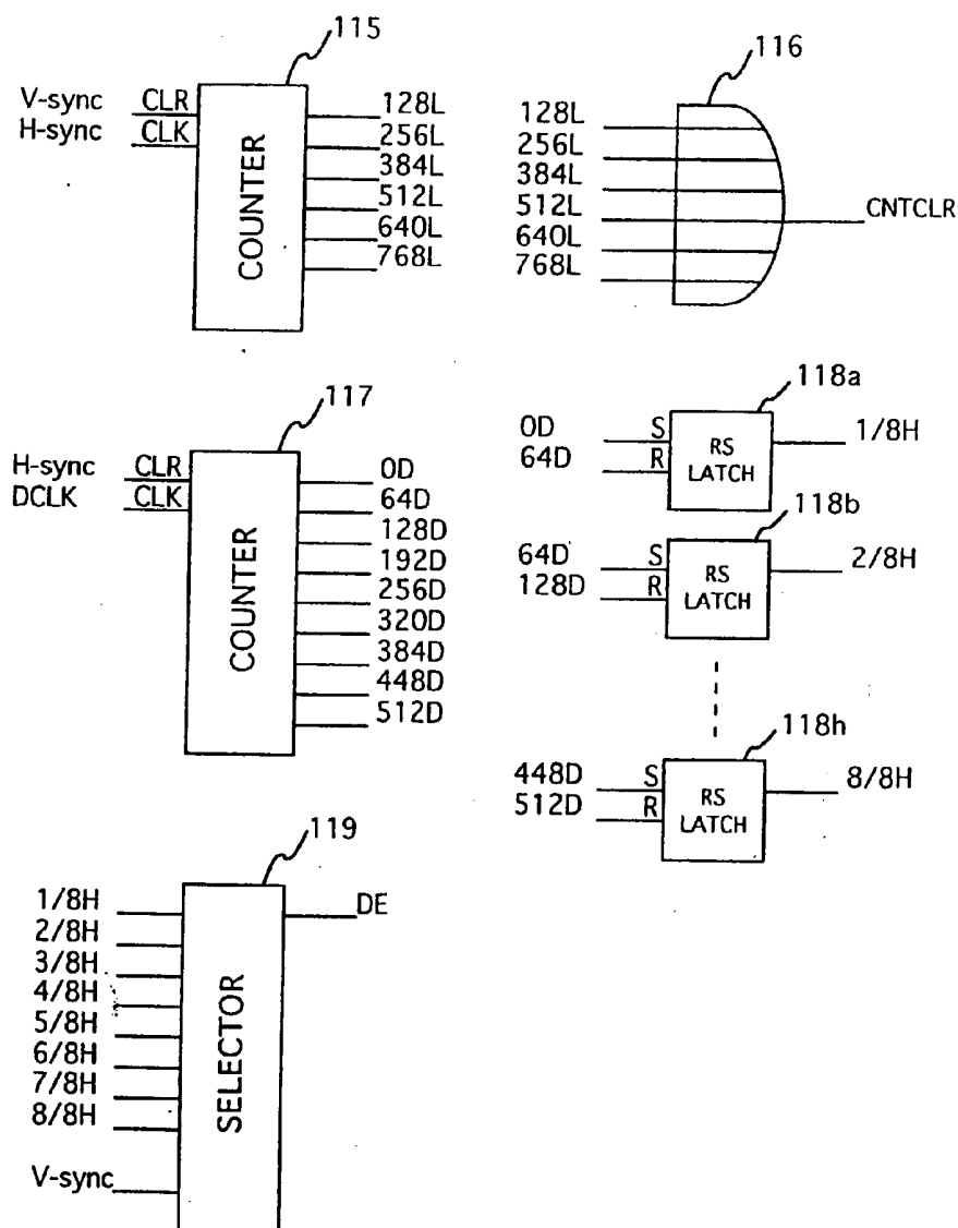
FIG. 40 DYNAMIC RANGE DESIGNATING PORTION
