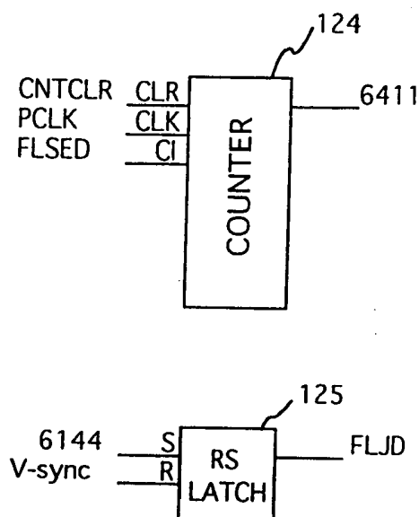
FIG. 42 FLICKER INFORMATION STORING PORTION
