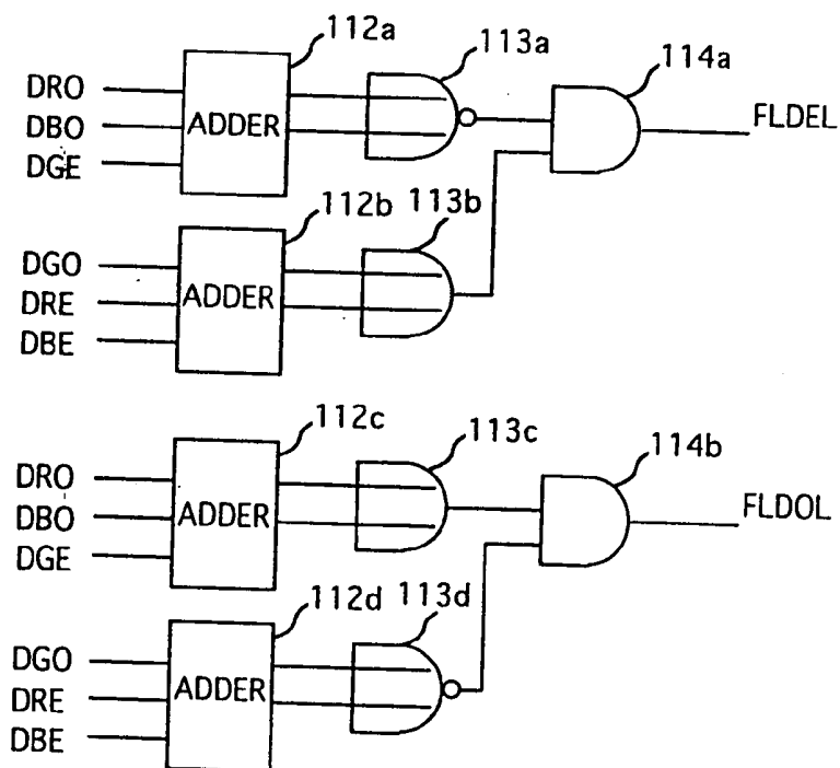
FIG. 39 FLICKER PATTERN DETECTING
