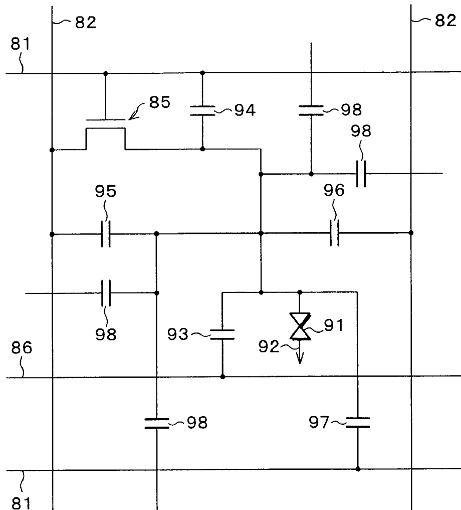
FIG. 11 (PRIOR ART)
