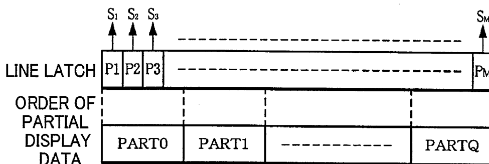
FIG. 12A SHL = "H"
