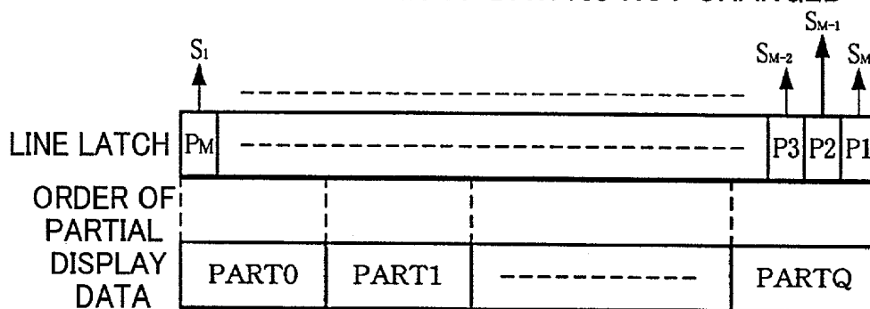
FIG. 12B SHL = "L" ORDER OF DATA IS NOT CHANGED
