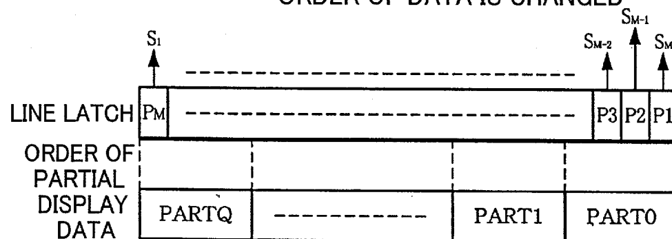
FIG. 12C SHL = "L" ORDER OF DATA IS CHANGED
