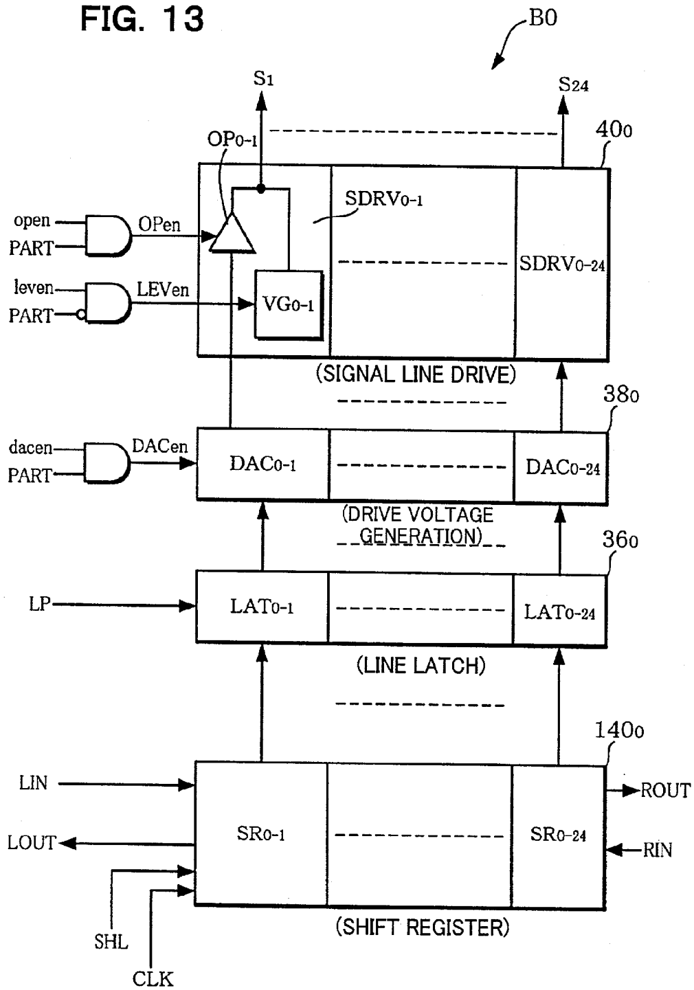
CONSTRUCTION OF SIGNAL DRIVER (AT BLOCK UNIT)
