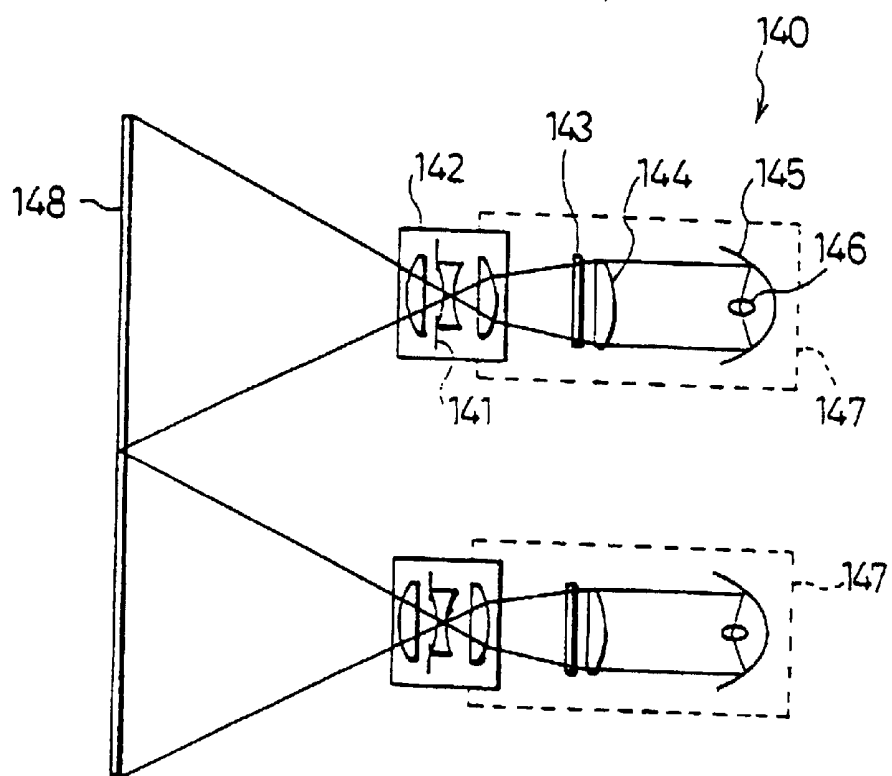
FIG. 18 (PRIOR ART)
