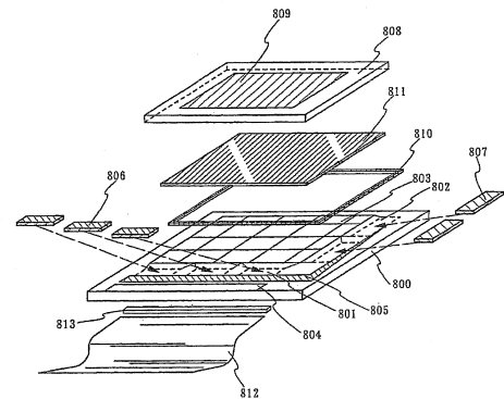
800: first substrate, 801: region for attaching a scanning line side IC chip, 802: region for attaching a data line side IC chip, 803: pixel region, 804: input-output terminal, 805: connecting wiring, 806, 807: IC chip, 808: second substrate, 809: opposing electrode, 810: sealing material, 811: liquid crystal, 812: FPC, 813: reinforcing plate
