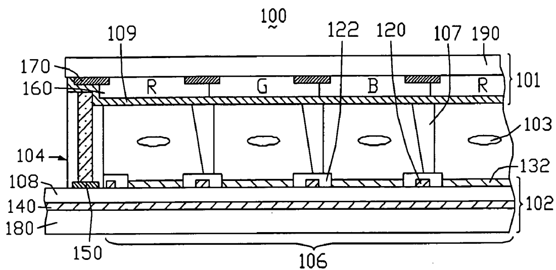
FIG. 7 (RELATED ART)
