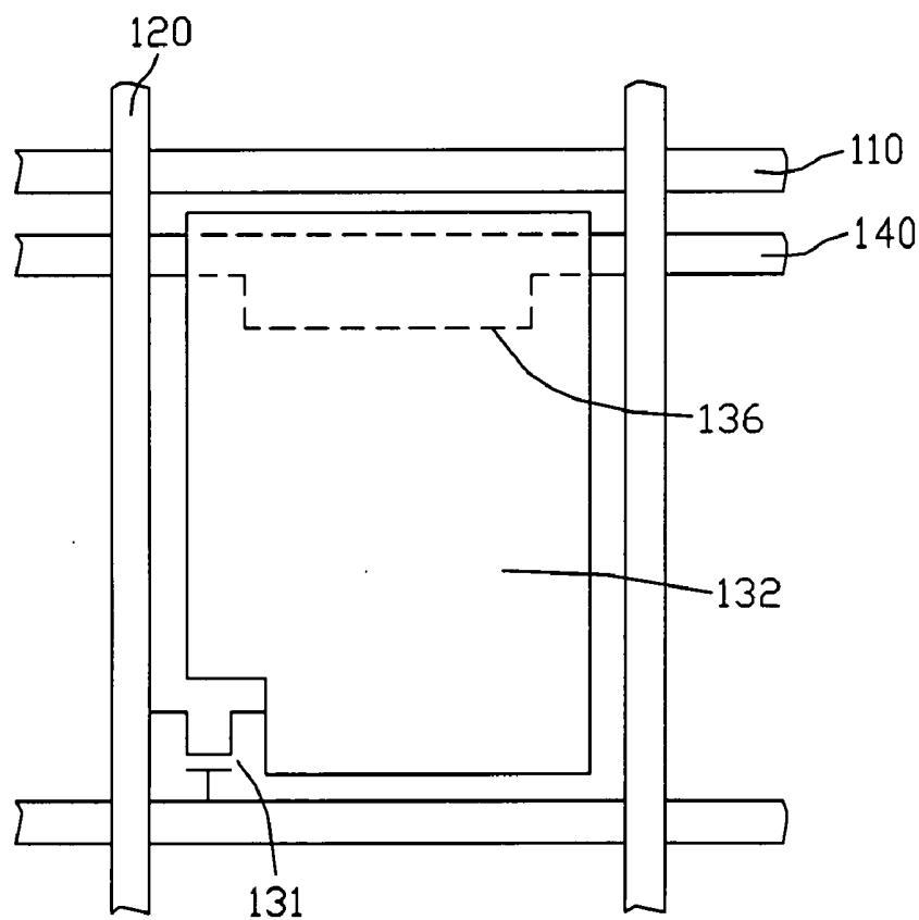
FIG. 8 (RELATED ART)
