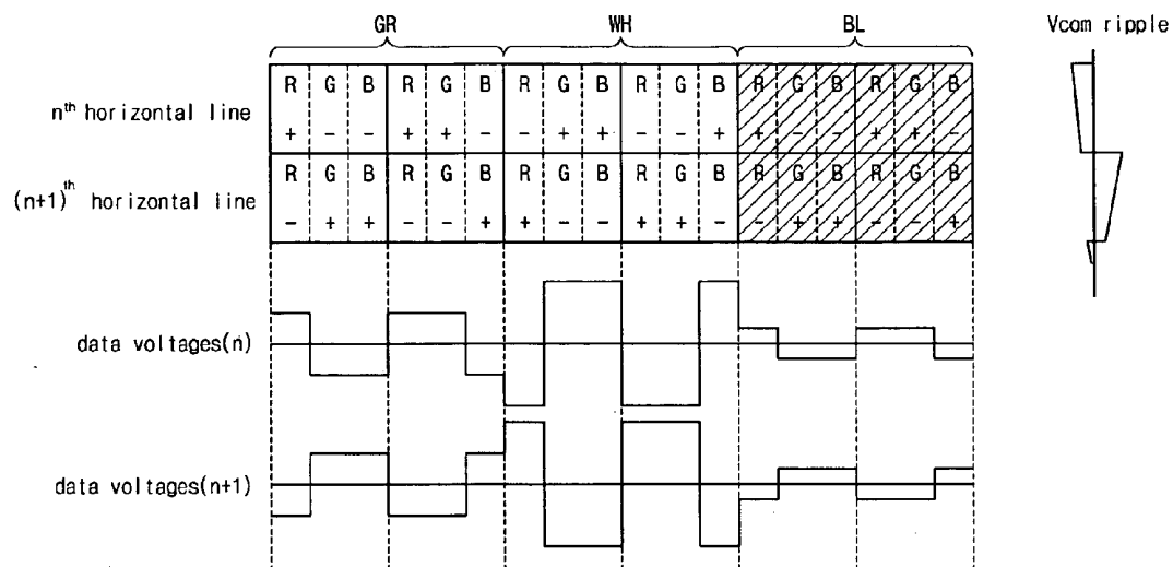
FIG. 4 RELATED ART
