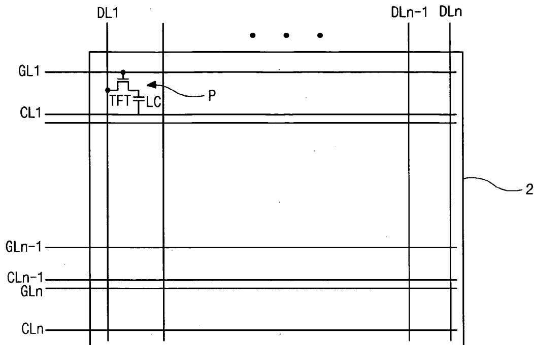
FIG. 2 RELATED ART
