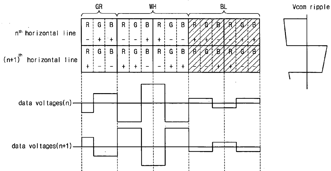
FIG. 3 RELATED ART
