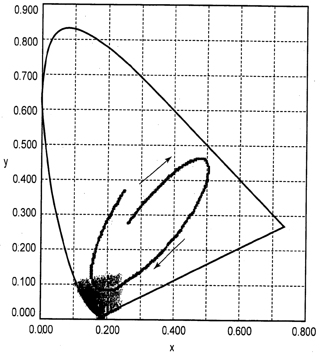
CHROMATICITY DIAGRAM
