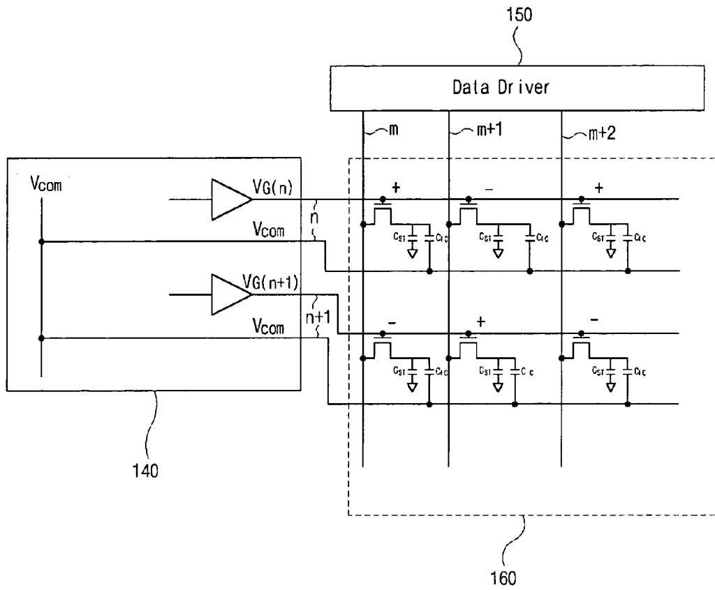
FIG. 2A (Related Art)
