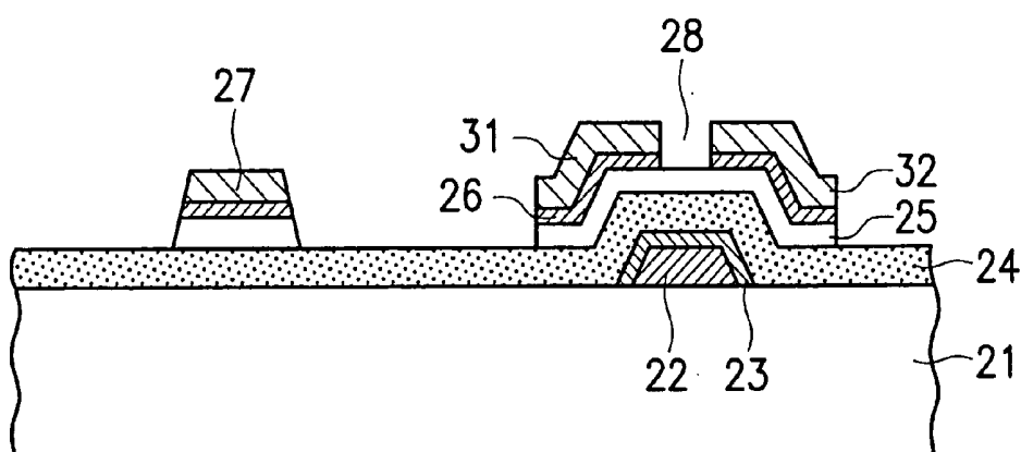
FIG. 1C (PRIOR ART)
