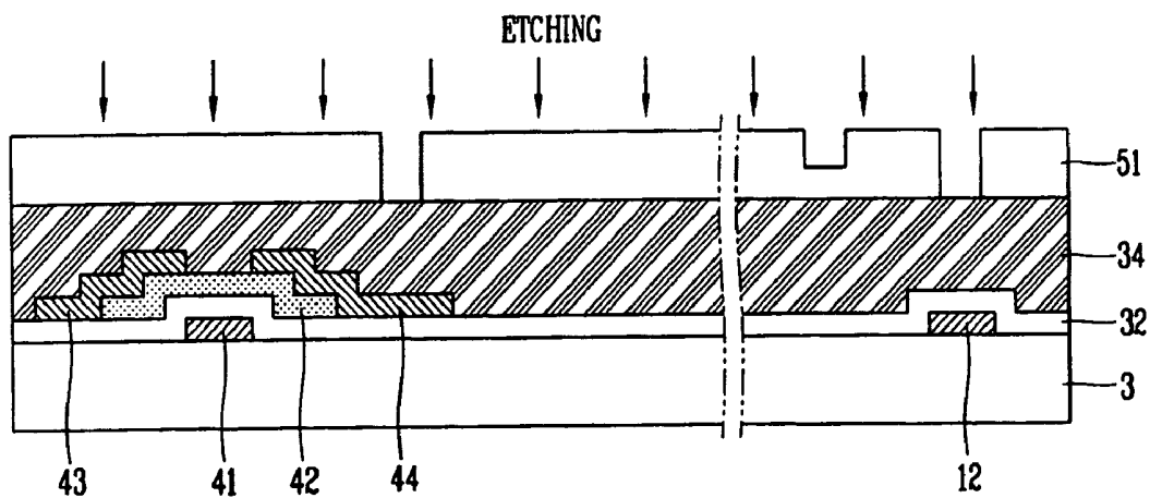
FIG. 2C RELATED ART
