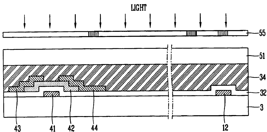
FIG. 2C RELATED ART
