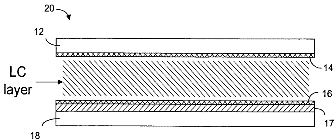
FIG.3 (prior art)
