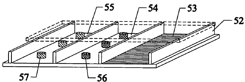
Fig.5c (PRIOR ART)
