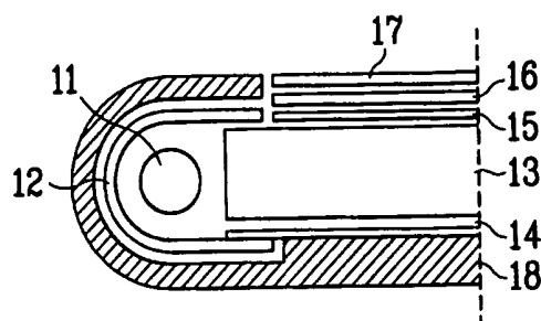
FIG. 3 Related Art
