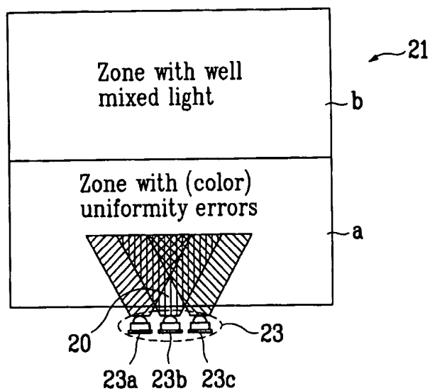
FIG. 4 Related Art
