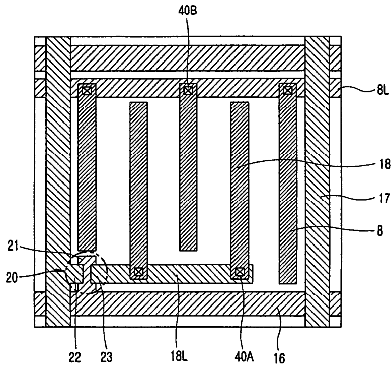
FIG. 1 RELATED ART
