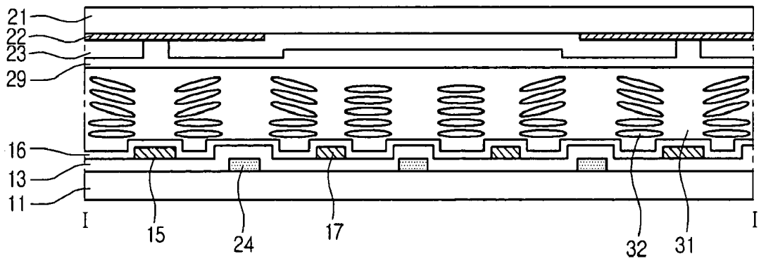
Fig.2 Related Art
