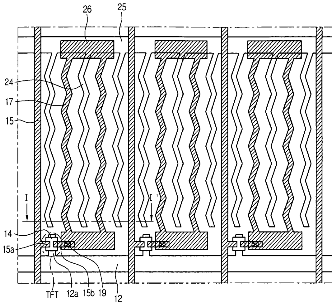
Fig.1 Related Art
