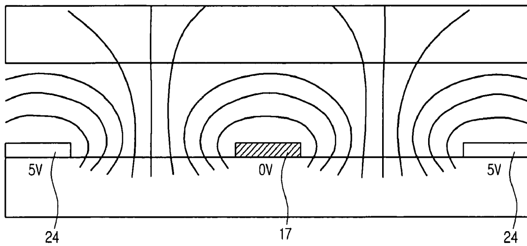
Fig.3 Related Art
