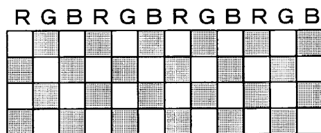
EVEN-NUMBERED FRAME
