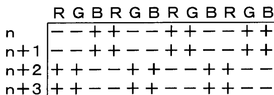
(4m+3)TH FRAME
