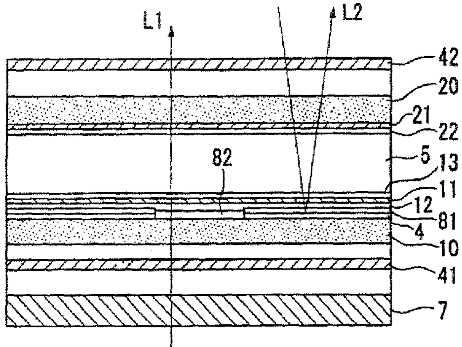
FIG. 9 (PRIOR ART)
