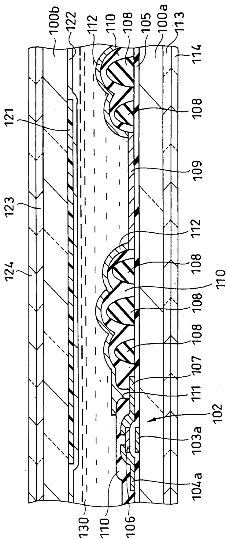
FIG. 2 (PRIOR ART)
