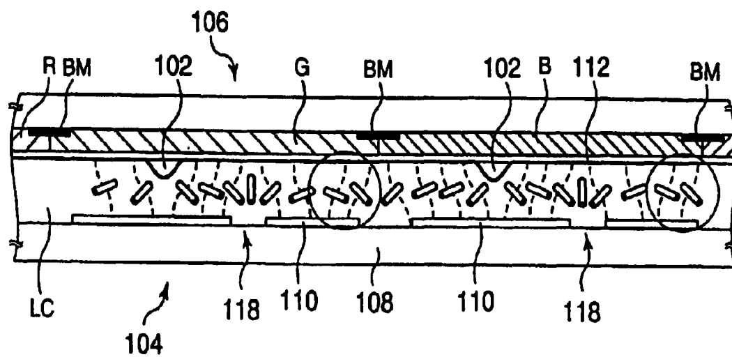
PRIOR ART FIG. 40
