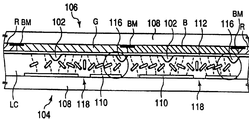
PRIOR ART FIG.42
