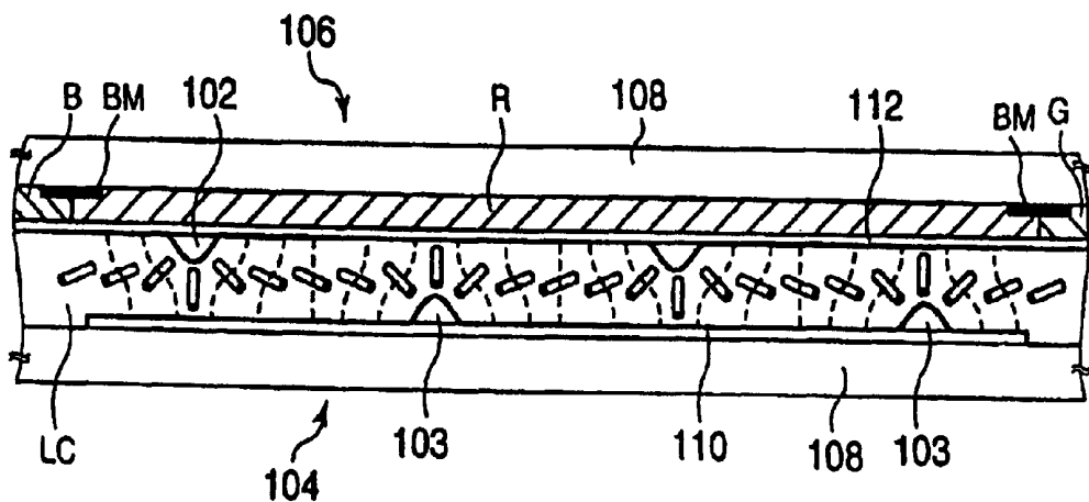
PRIOR ART FIG.38
