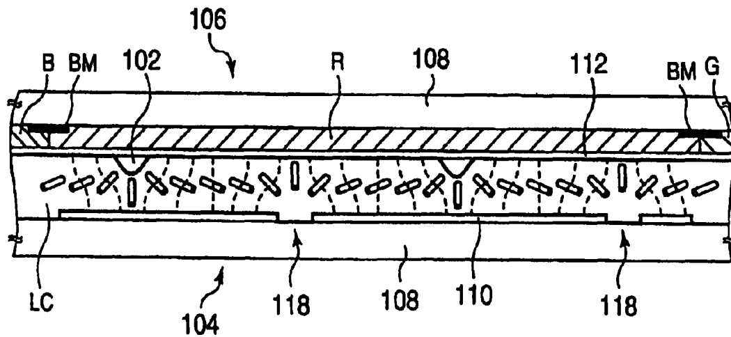
PRIOR ART FIG. 39
