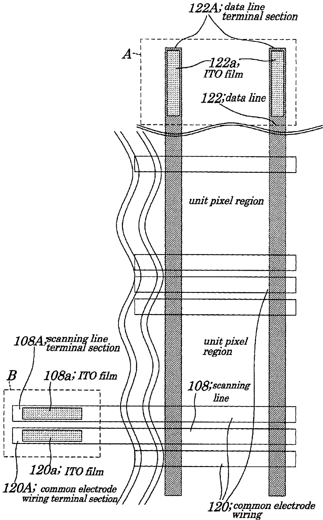
FIG. 40 (prior art)
