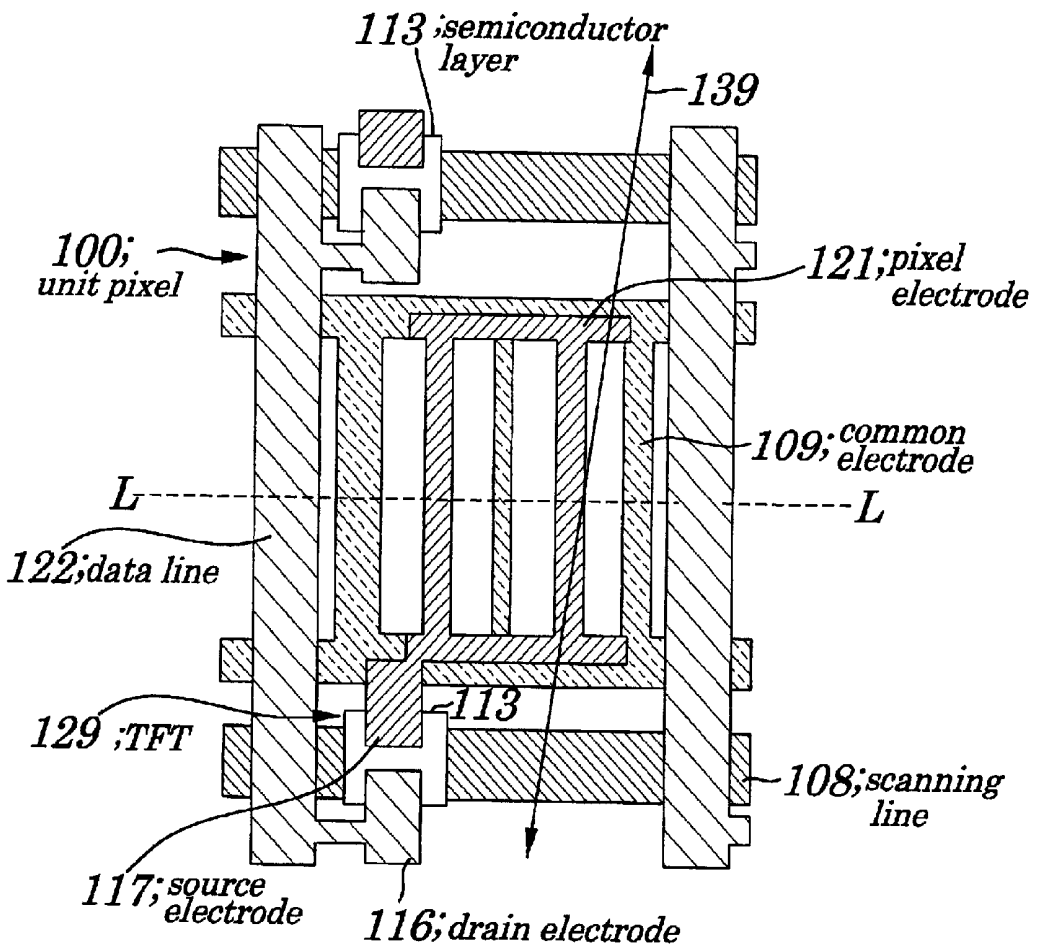
FIG.35 (prior art)
