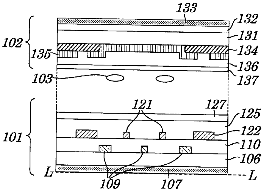
FIG.36 (prior art)
