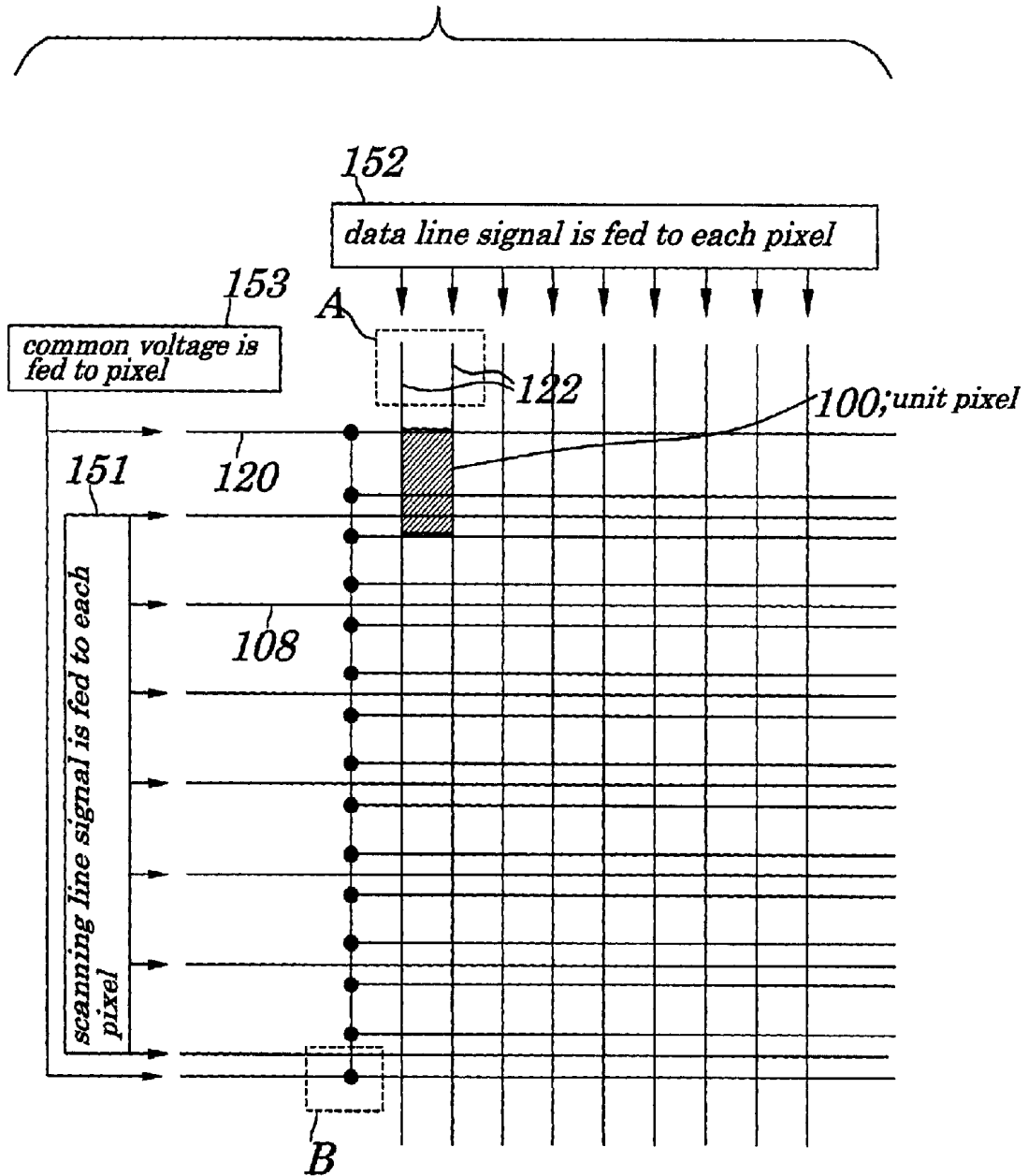
FIG. 39 (prior art)
