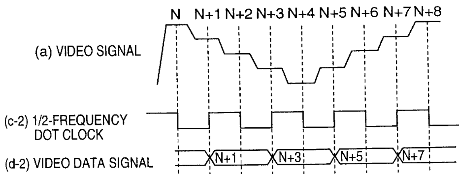
(2) ODD-NUMBER DOT DATA INPUT
