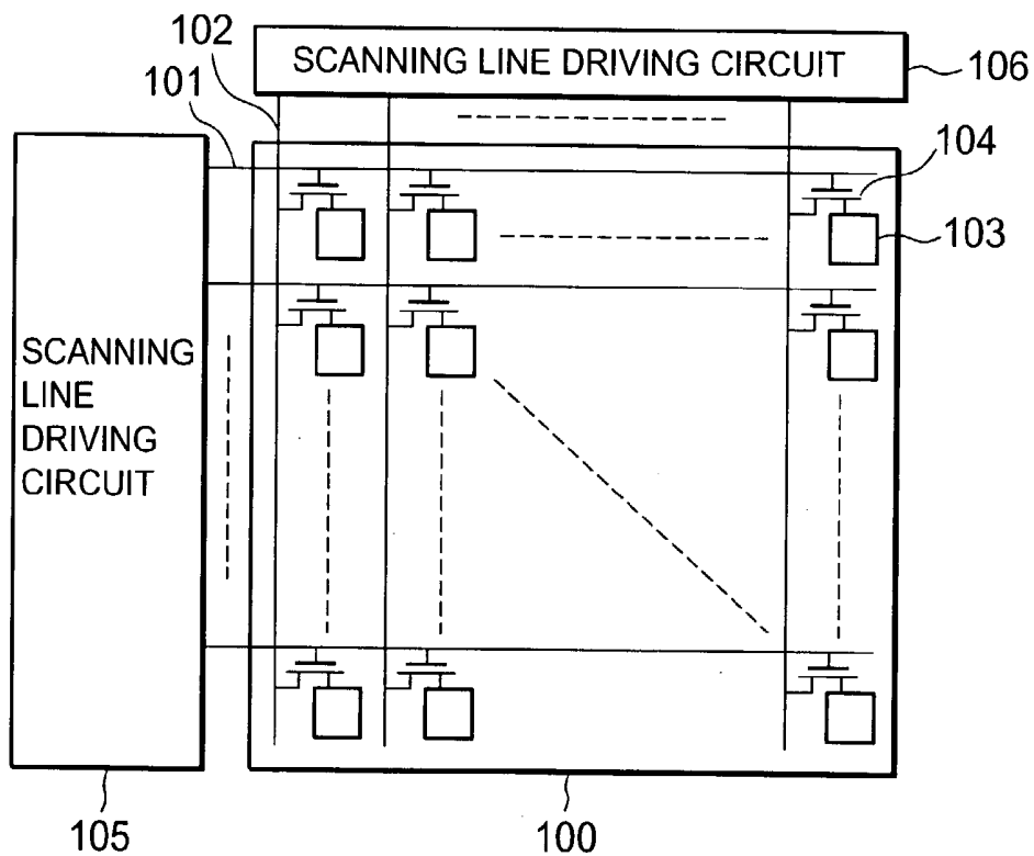
FIG. 6 (PRIOR ART)
