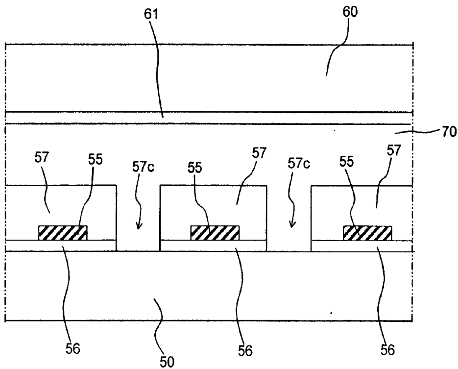
(related art) FIG. 3B
