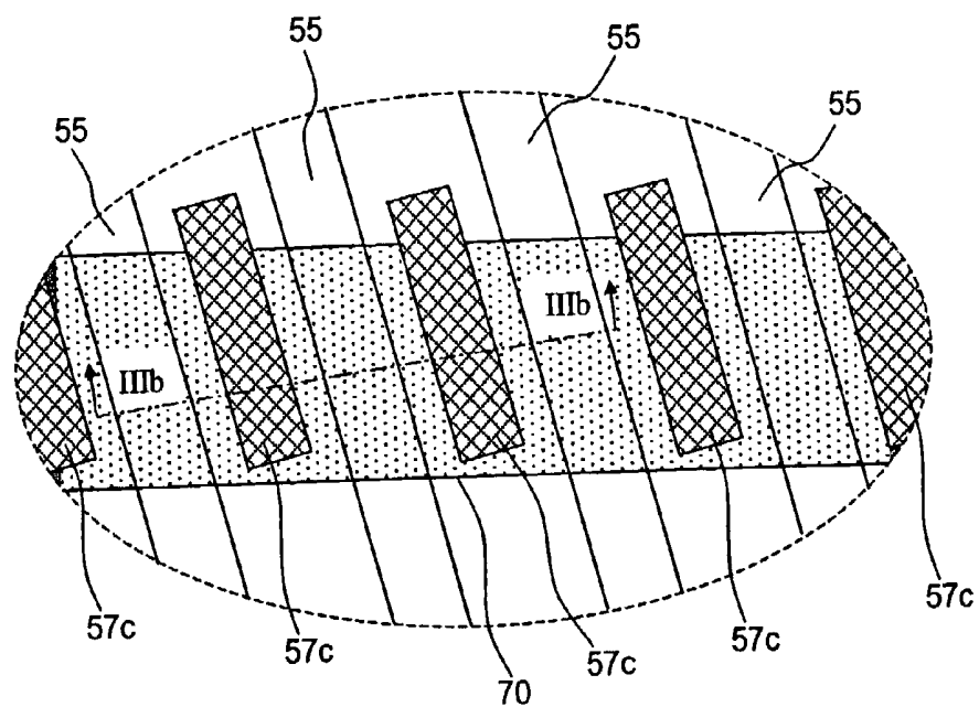
(related art) FIG. 3A
