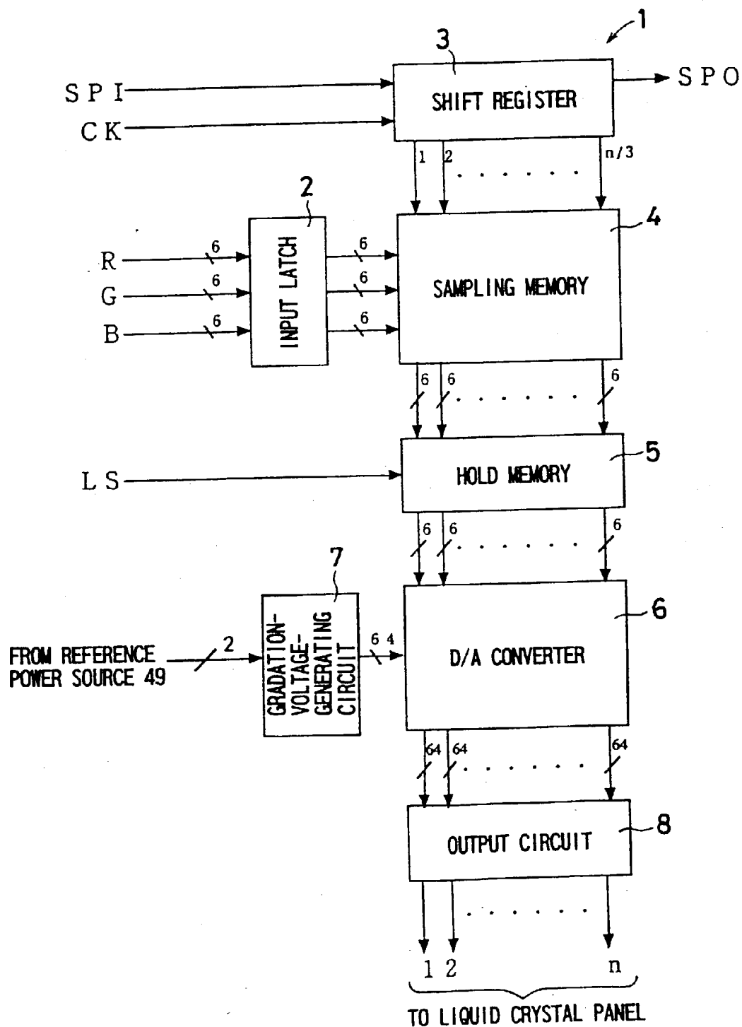
FIG. 10 PRIOR ART
