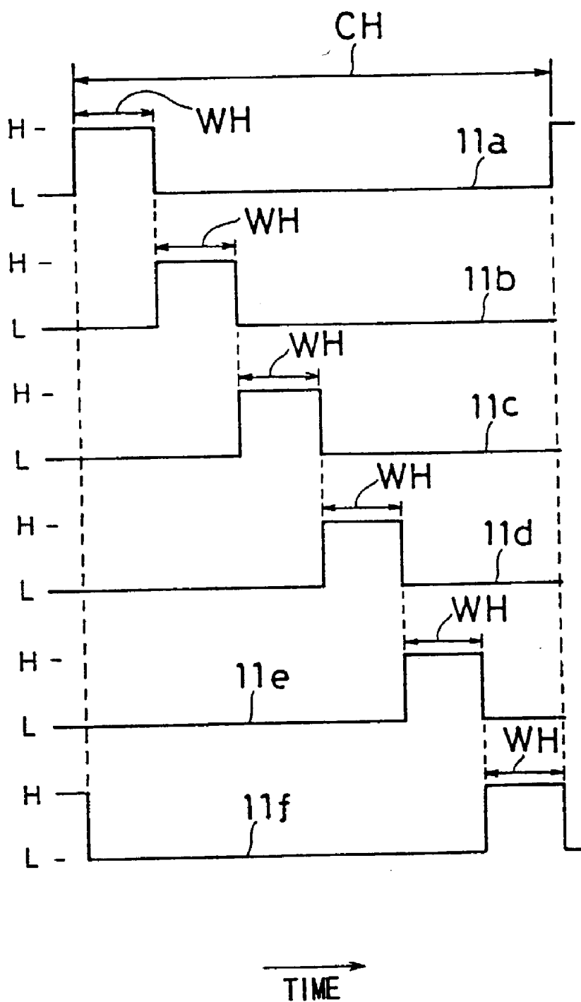
FIG. 11 PRIOR ART
