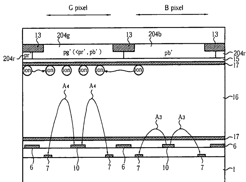
Fig. 10 Prior art
