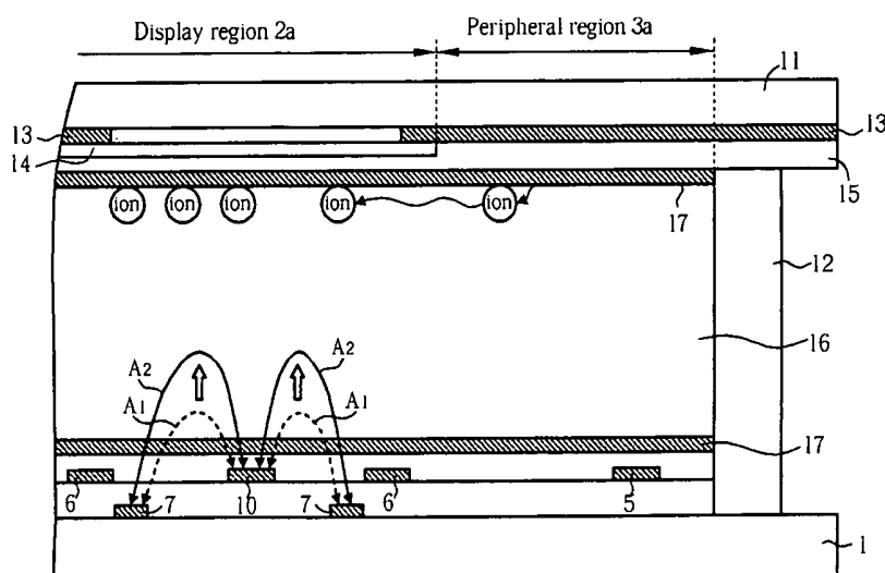
Fig. 4 Prior art
