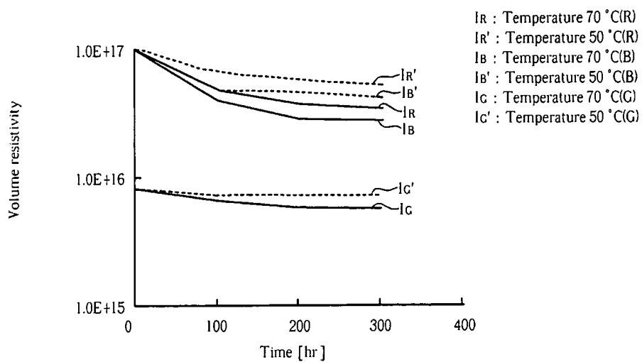
Fig. 9 Prior art
