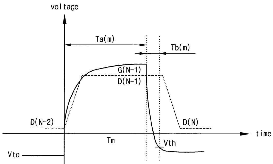
(related art) FIG. 4B
