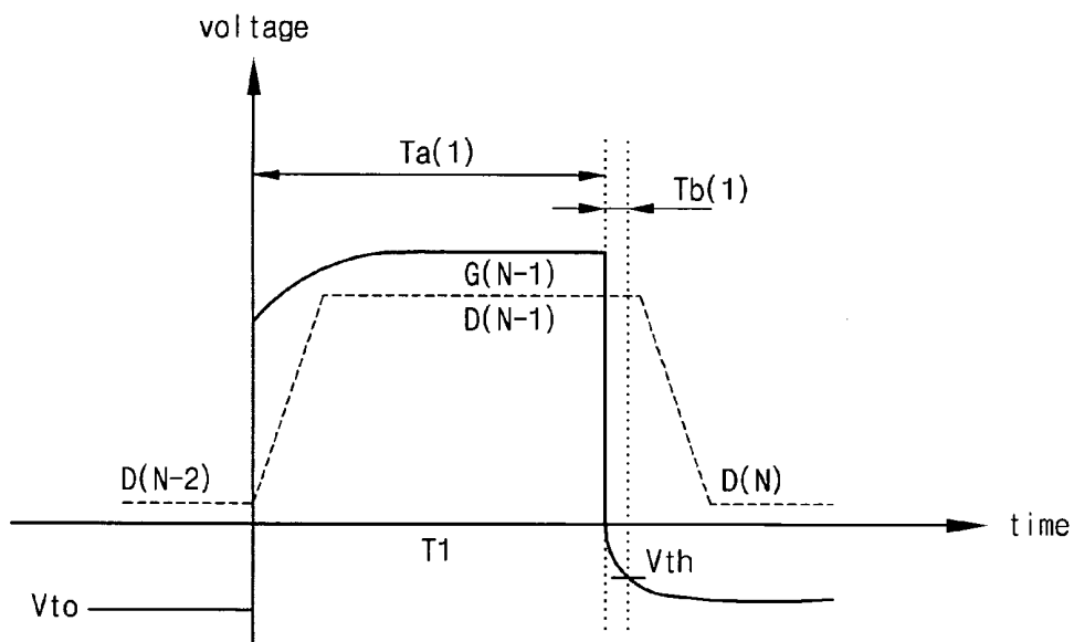
(related art) FIG. 4A
