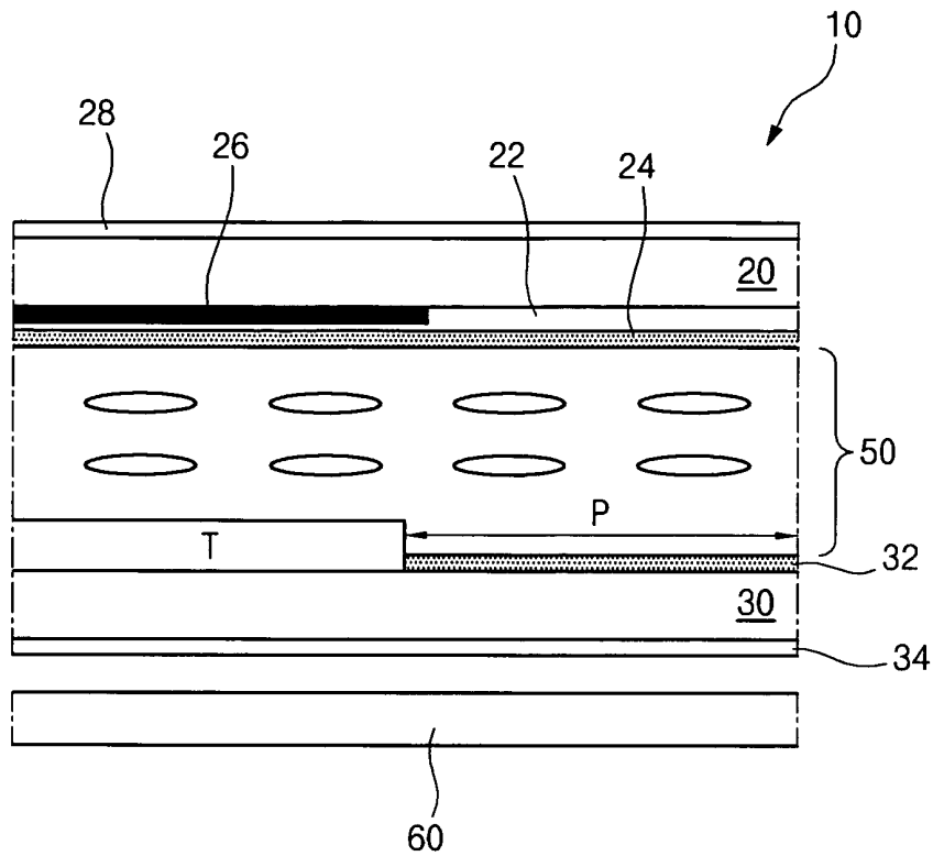
(related art) FIG. 1
