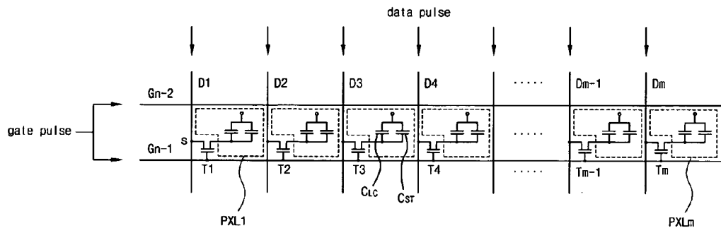
(related art) FIG. 3
