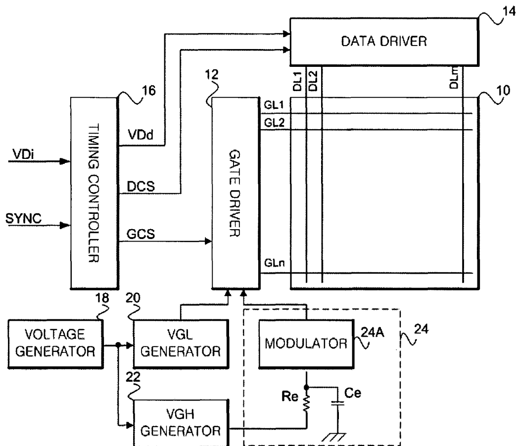
Fig. 2 (Related Art)
