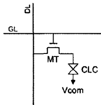
Fig. 2 (Related Art)
