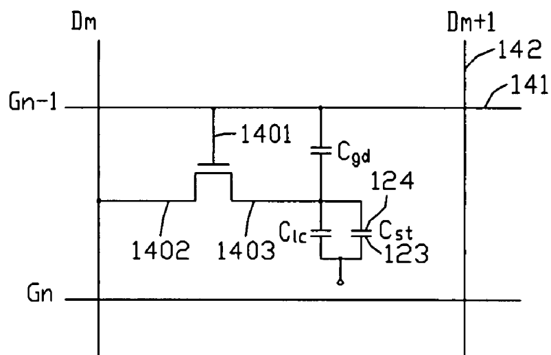
FIG. 7 (RELATED ART)
