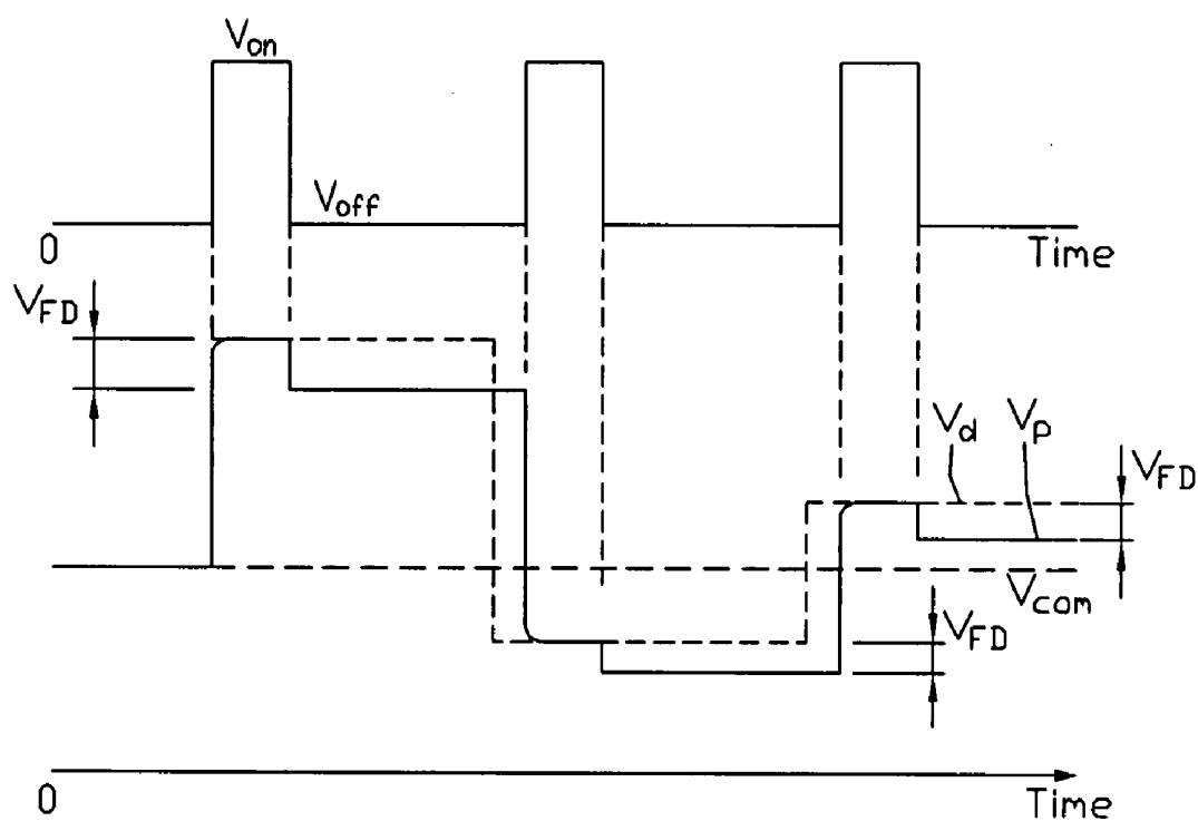
FIG. 8 (RELATED ART)
