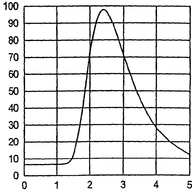
\Delta nd=0.29 REFLECTION CHARACTERISTIC (VERTICAL AXIS: REFLECTANCE (%), HORIZONTAL AXIS : VOLTAGE (V))
