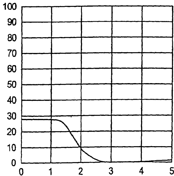
\Delta nd=0.15 TRANSMISSION CHARACTERISTIC (VERTICAL AXIS: REFLECTANCE (%), HORIZONTAL AXIS : VOLTAGE (V))
