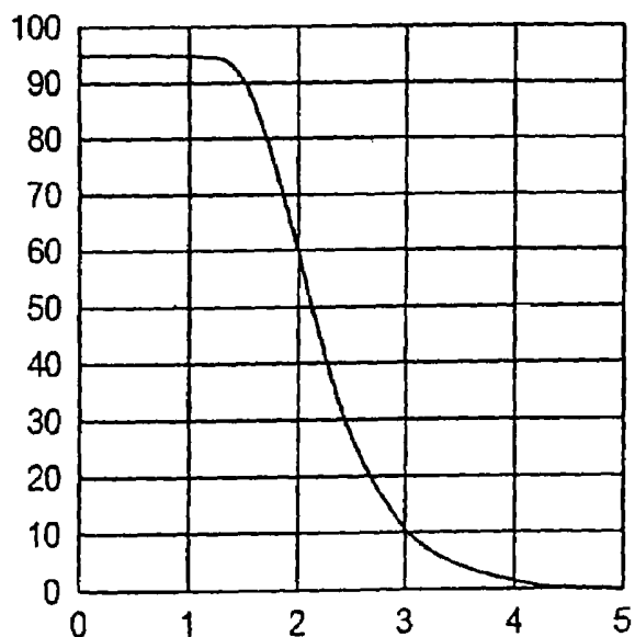
\Delta nd=0.29 TRANSMISSION CHARACTERISTIC (VERTICAL AXIS: REFLECTANCE (%), HORIZONTAL AXIS : VOLTAGE (V))
