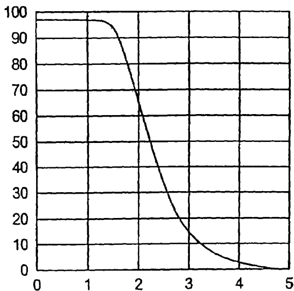
\Delta nd=0.15 REFLECTION CHARACTERISTIC (VERTICAL AXIS: REFLECTANCE (%), HORIZONTAL AXIS : VOLTAGE (V))
