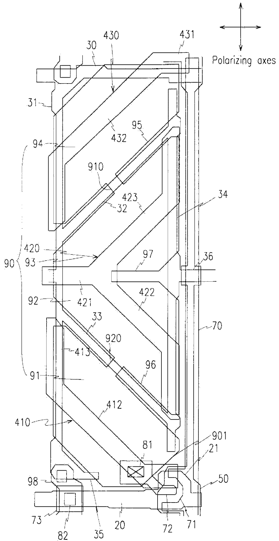
Fig.5C
