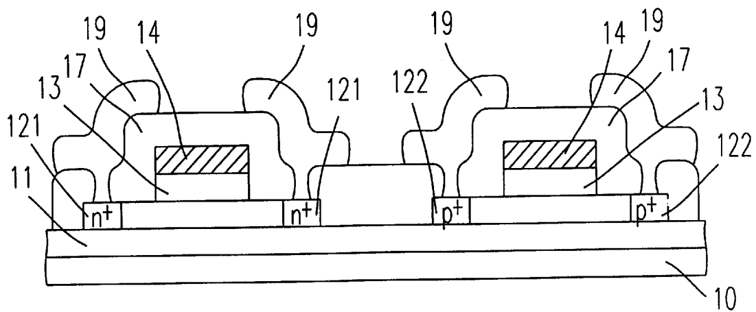
Fig. 1(f)(PRIOR ART)
