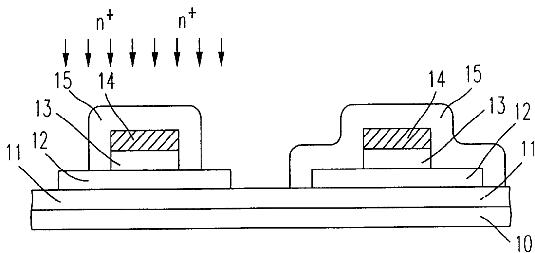
Fig. 1(c)(PRIOR ART)
