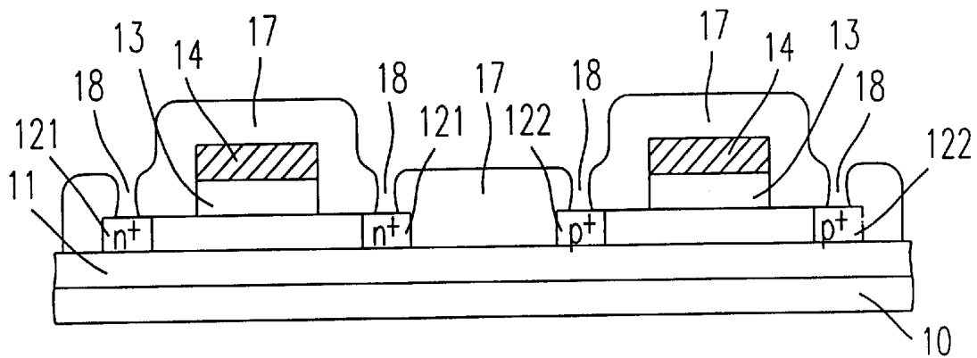
Fig. 1(e)(PRIOR ART)
