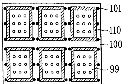
FIG. 2C Related Art
