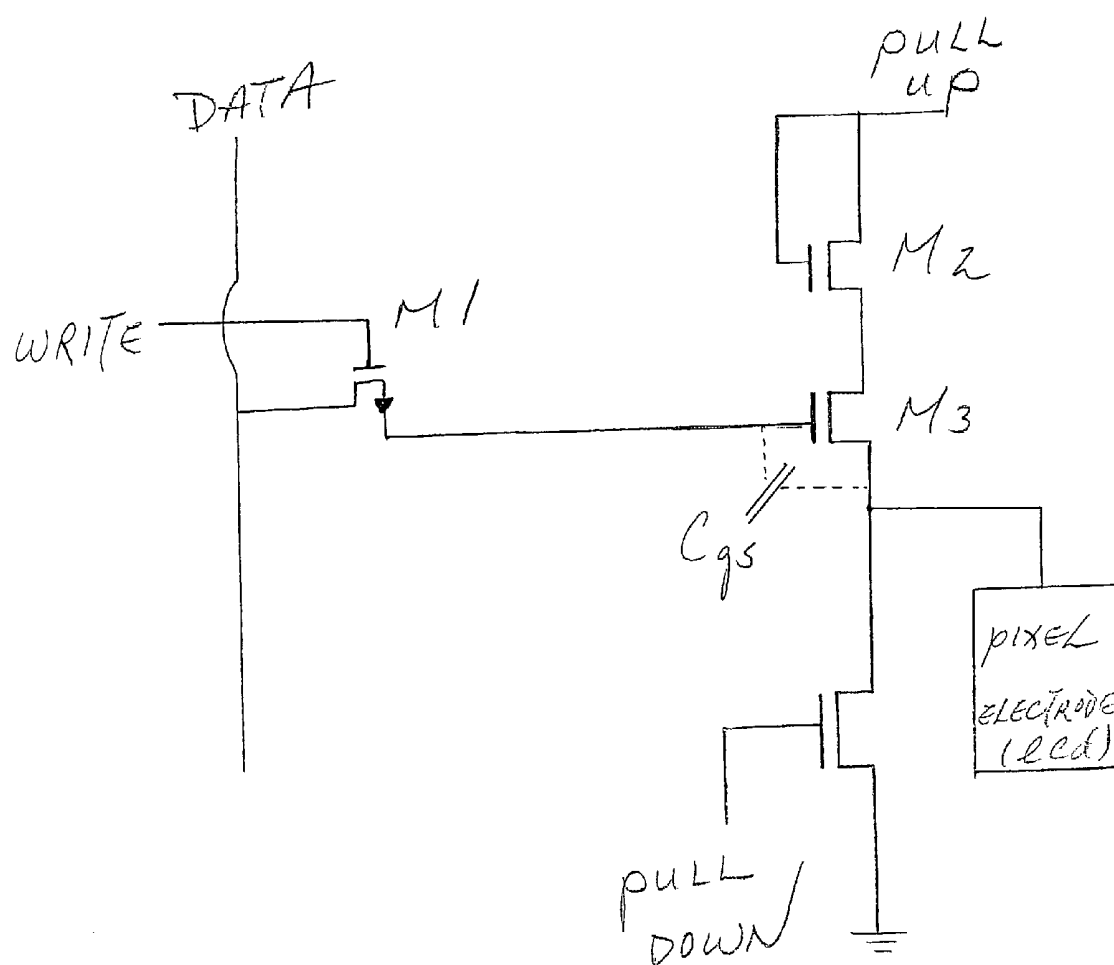
FIG. 4 FRAME BUFFER PIXEL BACKGROUND ART
