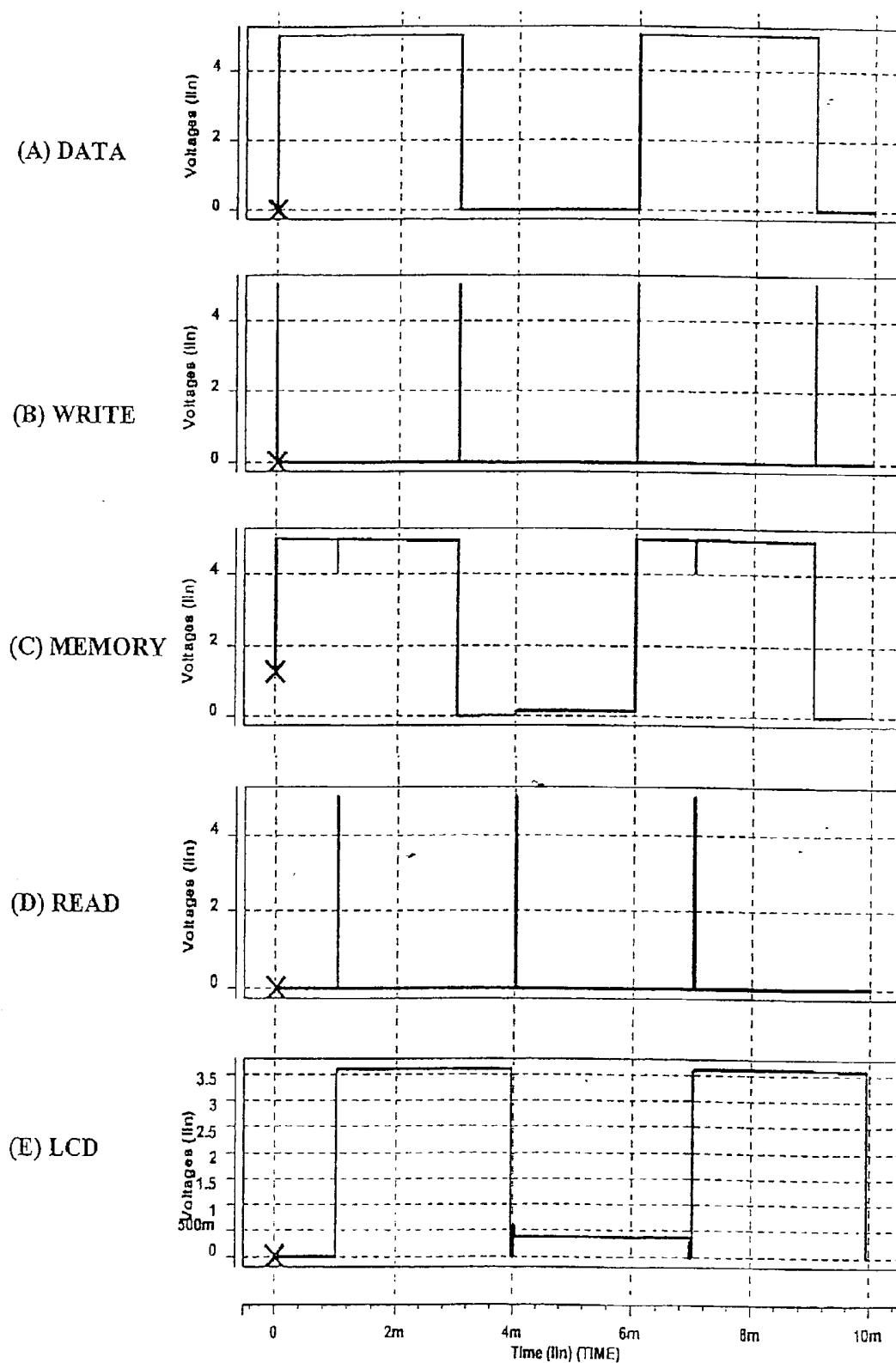
Figure 8. Hspice simulation results performed for Fig. 7 frame buffer pixel showing voltage levels at nodes with respect to time.
