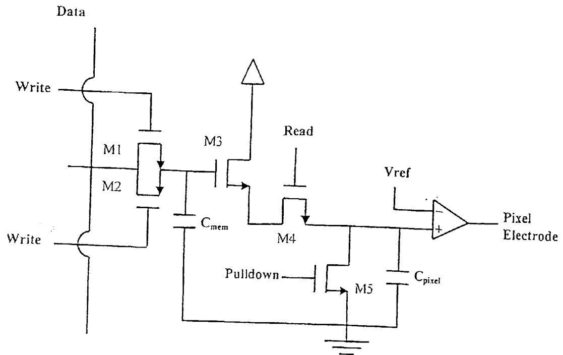
Figure 14 Frame buffer pixel with a comparator.
