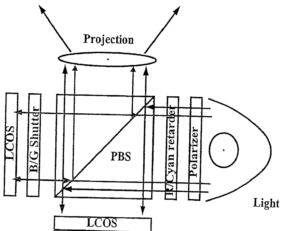
Figure 9 2-panel projection display with partial field sequential color.
