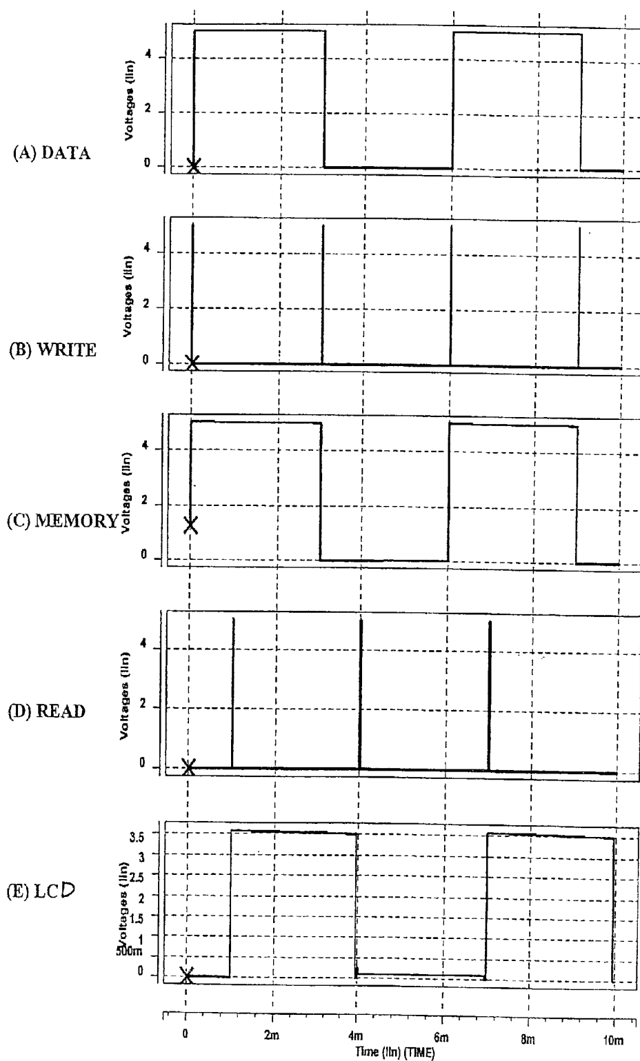
Figure 11 Hspice simulation results performed for the FIG. 10 frame buffer pixel ILLUSTRATING voltage levels at nodes with respect to time.
