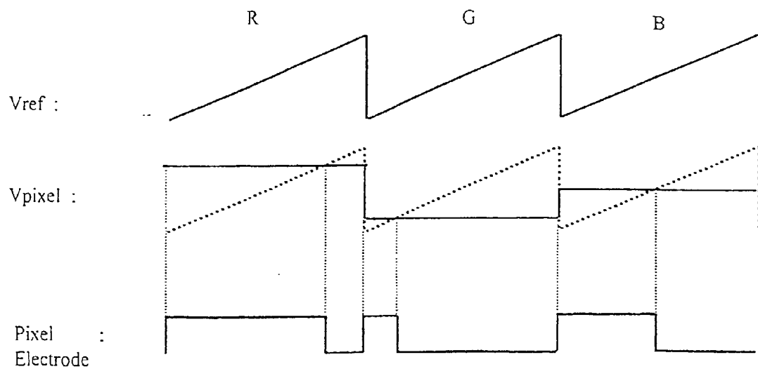
Figure 16 PWM waveform generated from the pixel voltage and reference voltage.
