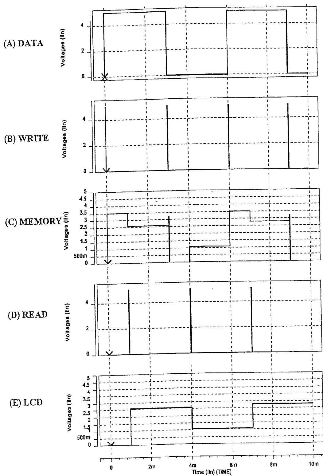
Figure 3 Hspice simulation results for the conventional frame buffer pixel display voltage levels at nodes with respect to time.
