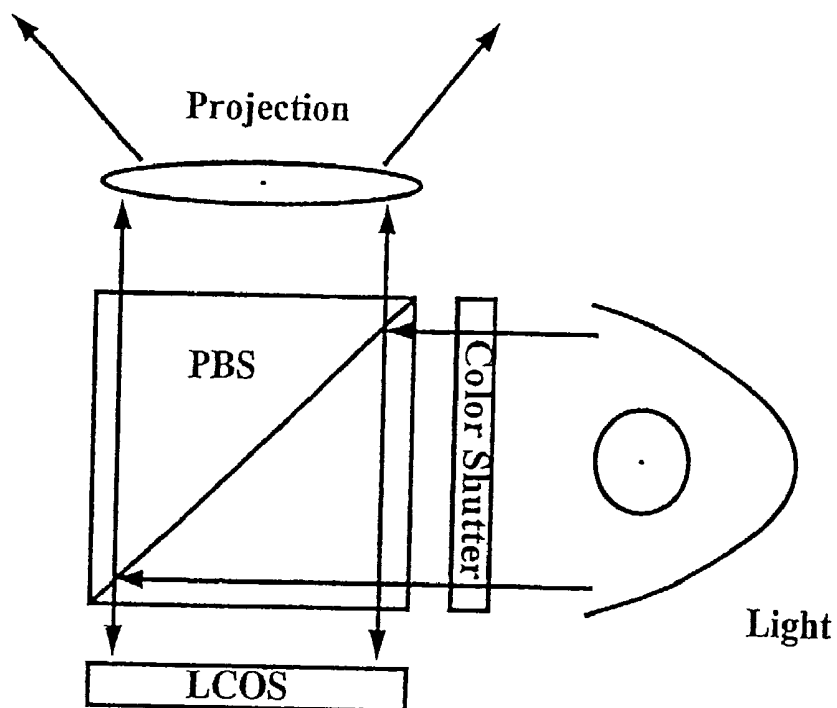
Figure 8 1-panel projection display with field sequential color.
