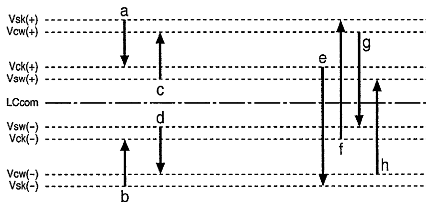
(A) D/A OPERATION
