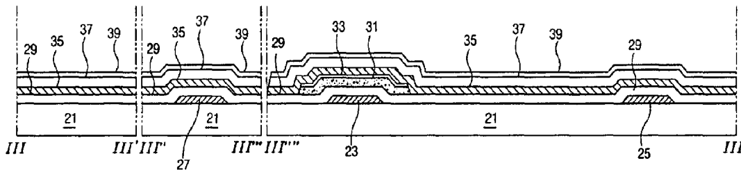
(related art) FIG. 4B
