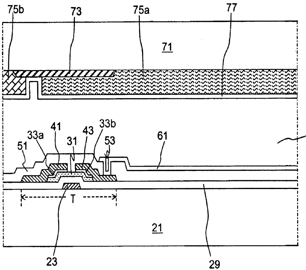
(related art) FIG. 1
