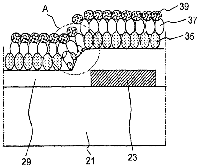
(related art) FIG. 5A
