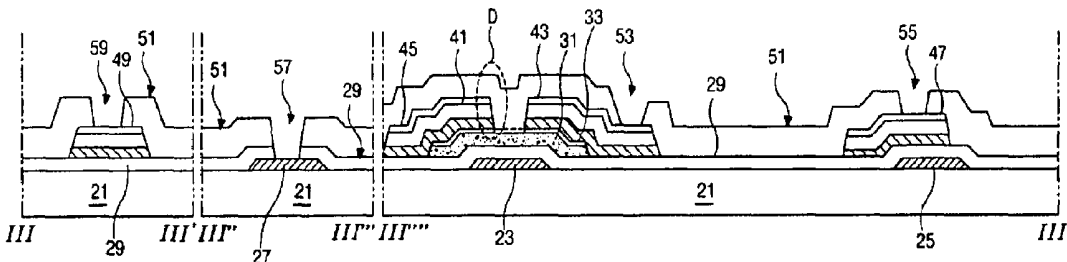
(related art) FIG. 4D
