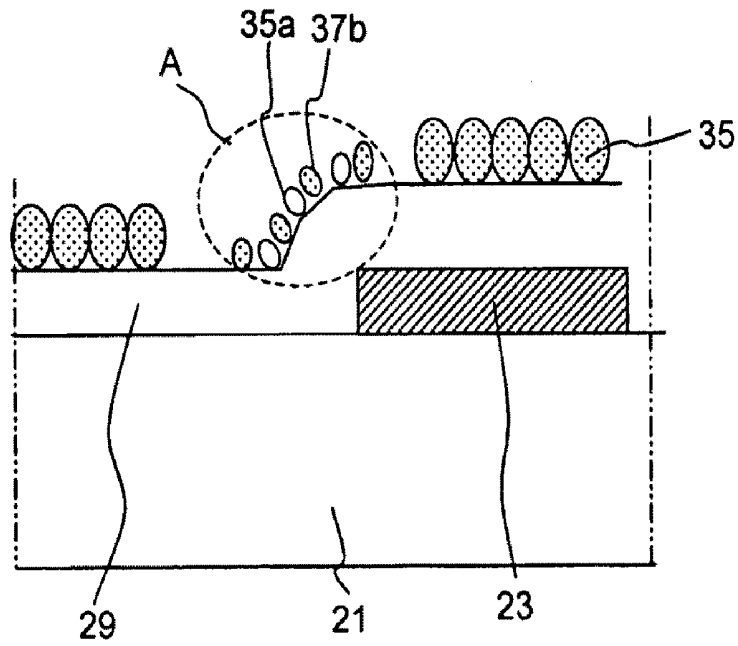
(related art) FIG. 5B
