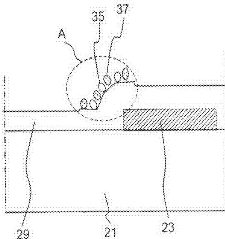
(related art) FIG. 5D
