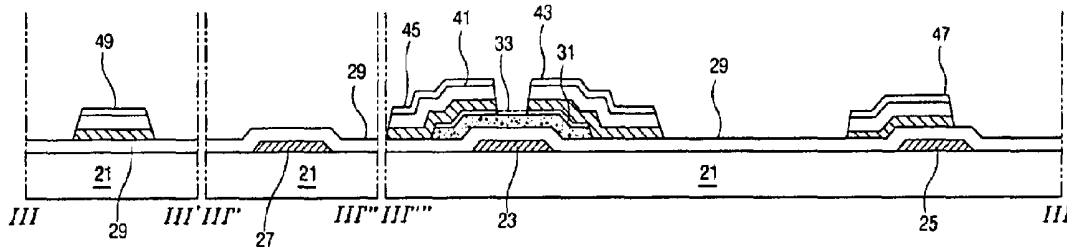
(related art) FIG. 4C
