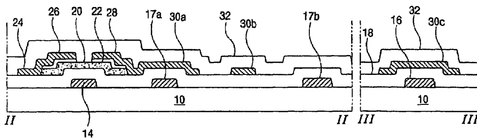
FIG. 2C (RELATED ART)
