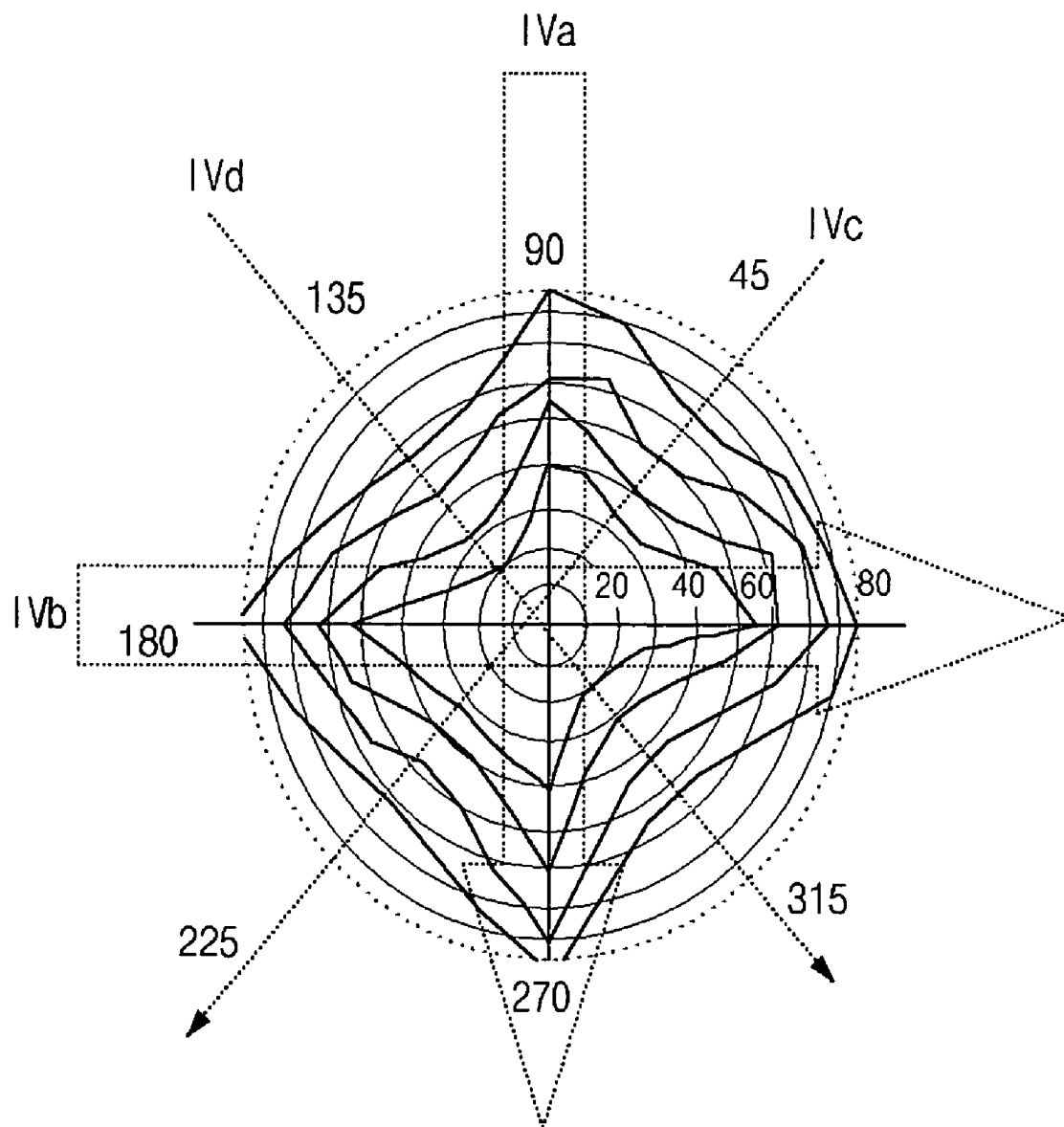
FIG. 4 (RELATED ART)
