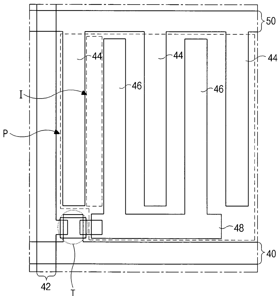
FIG. 2 (RELATED ART)
