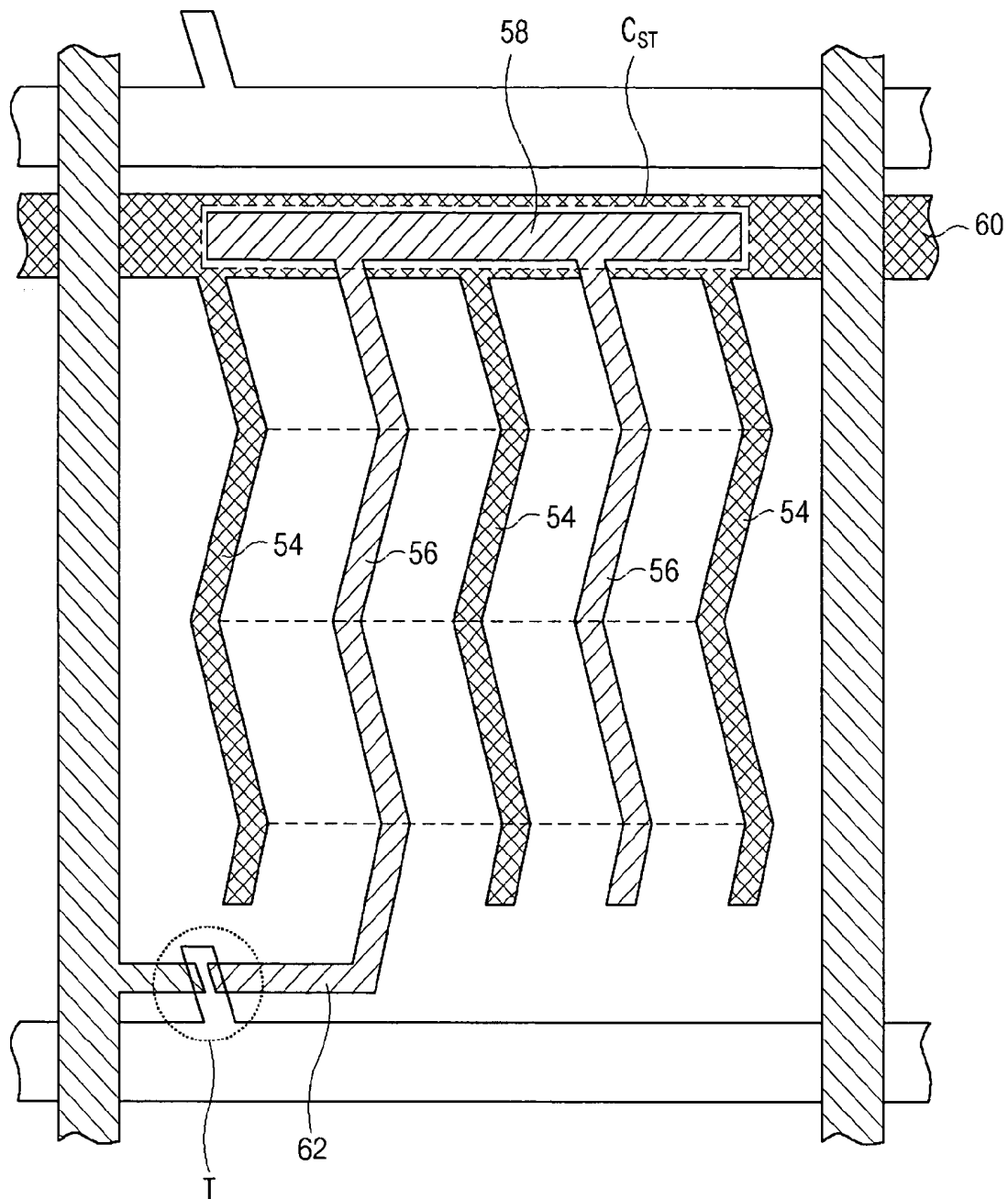
FIG. 3 (RELATED ART)
