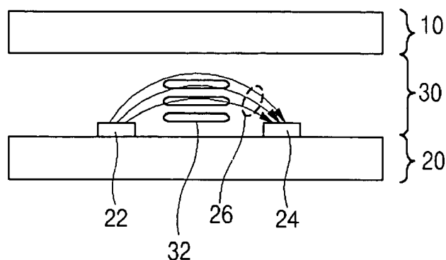
FIG. 1 (RELATED ART)
