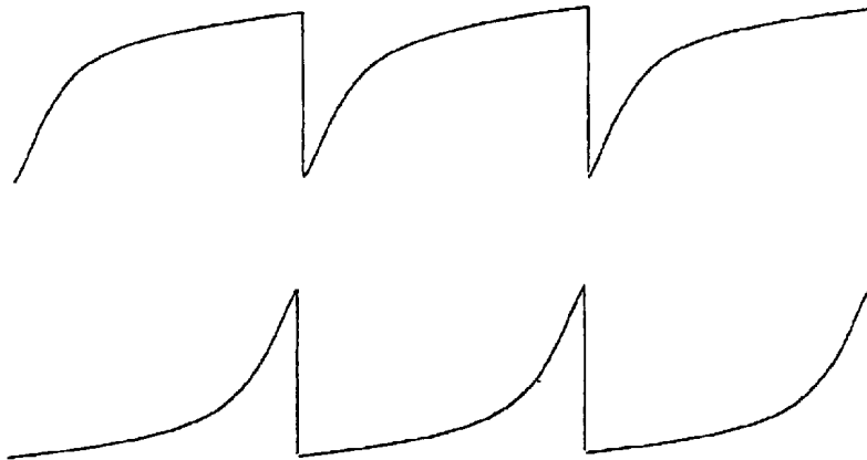
Figure 17 WAVEFORM OF THE REFERENCE VOLTAGE VARIED TO APPLY GAMMA CORRECTIONS.
