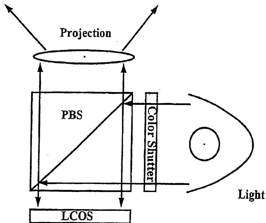
Figure 18 1-panel projection display with field sequential color.
