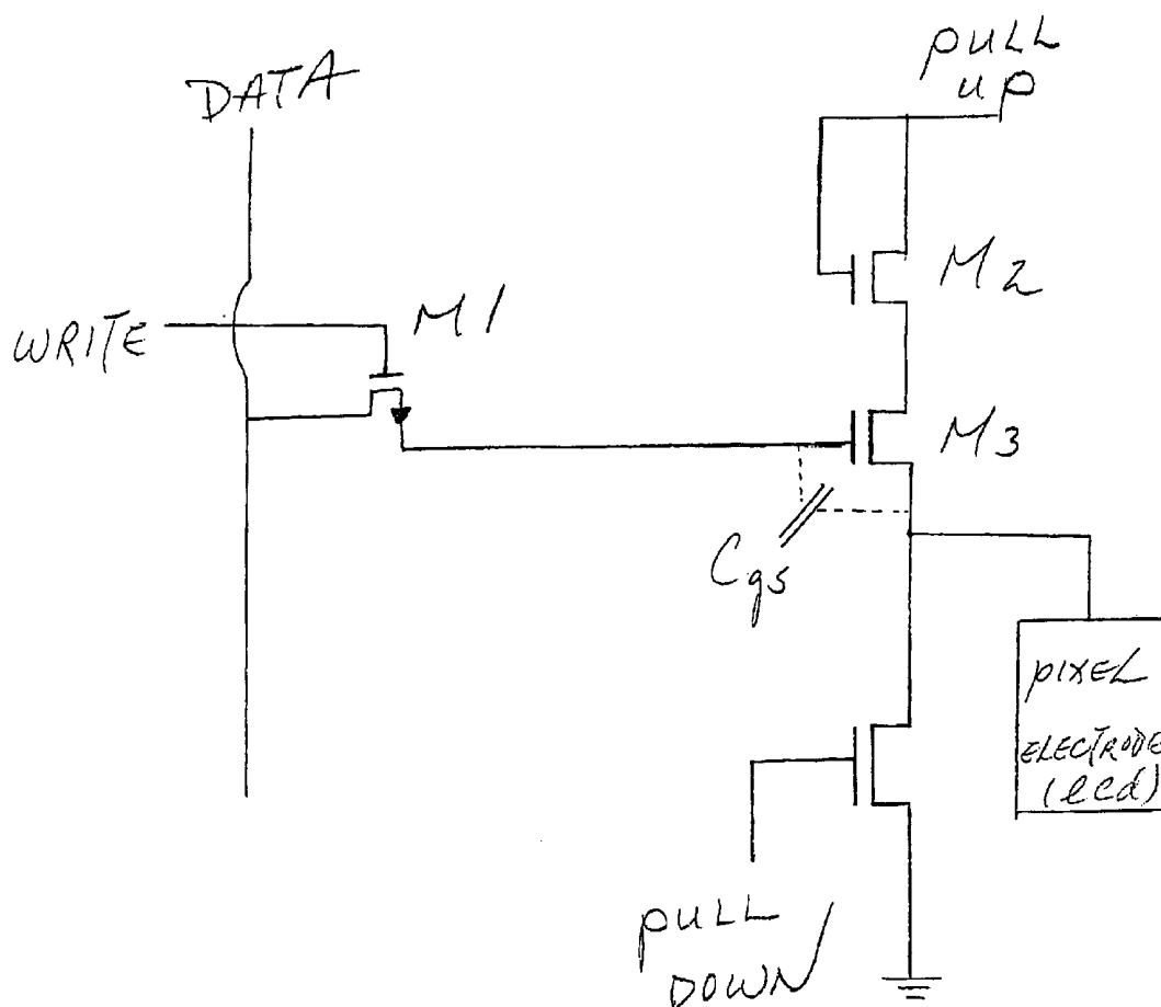
FIG. 4 BUFFER PIXEL FRAME BACKGROUND ART
