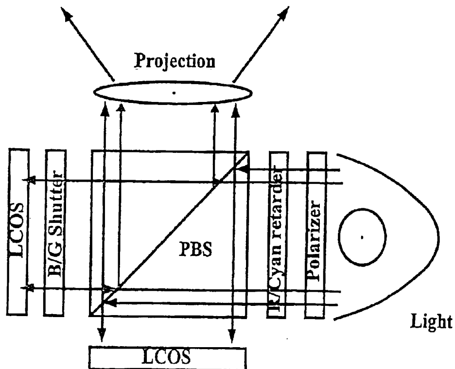
Figure 19 2-panel projection display with partial field sequential color.
