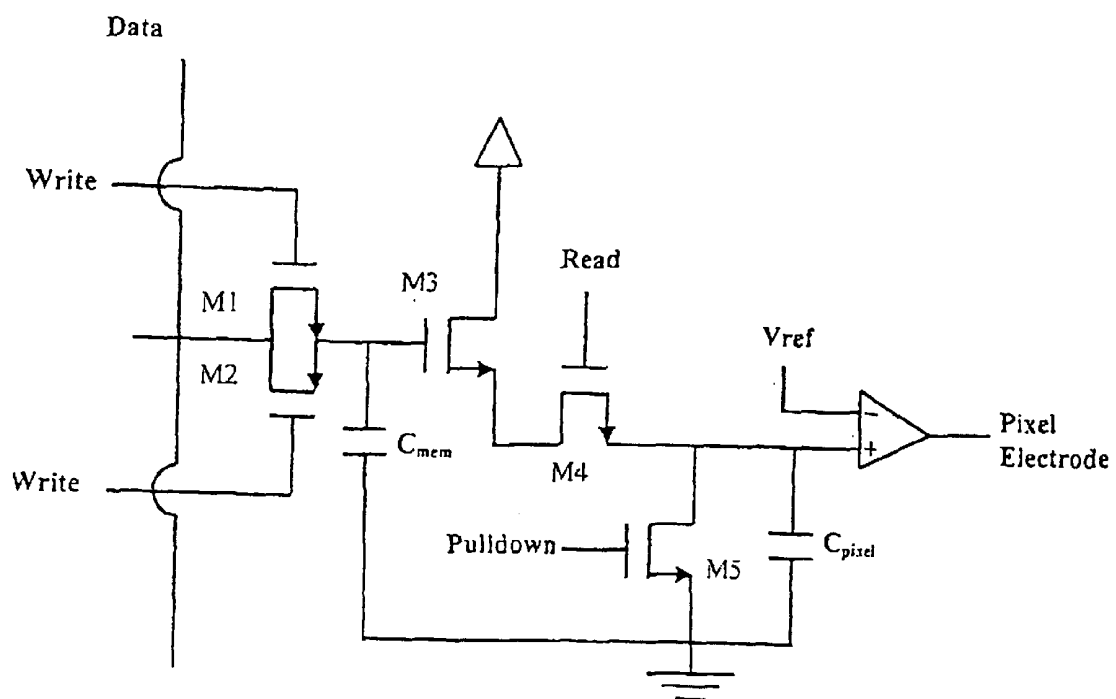
Figure: \mu Frame buffer pixel with a comparator.
