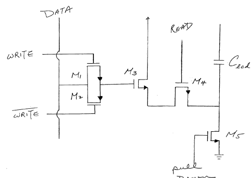
A REFINED FRAME BUFFER PIXEL CIRCUIT
