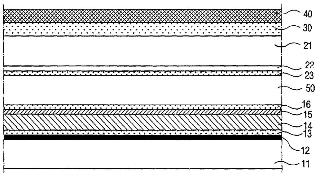
FIG. 2 (RELATED ART)
