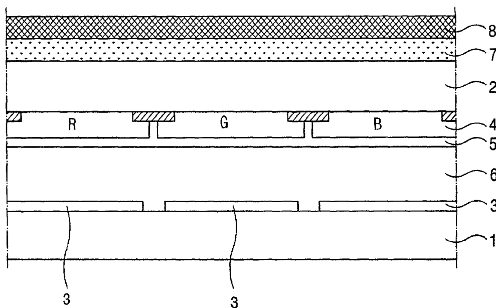
FIG. 1 (RELATED ART)
